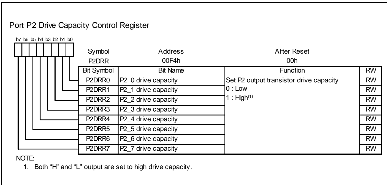
Figure 7.10 P2DRR Register
