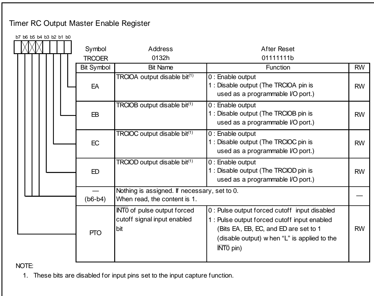
Figure 16.37 TRCOER Register
