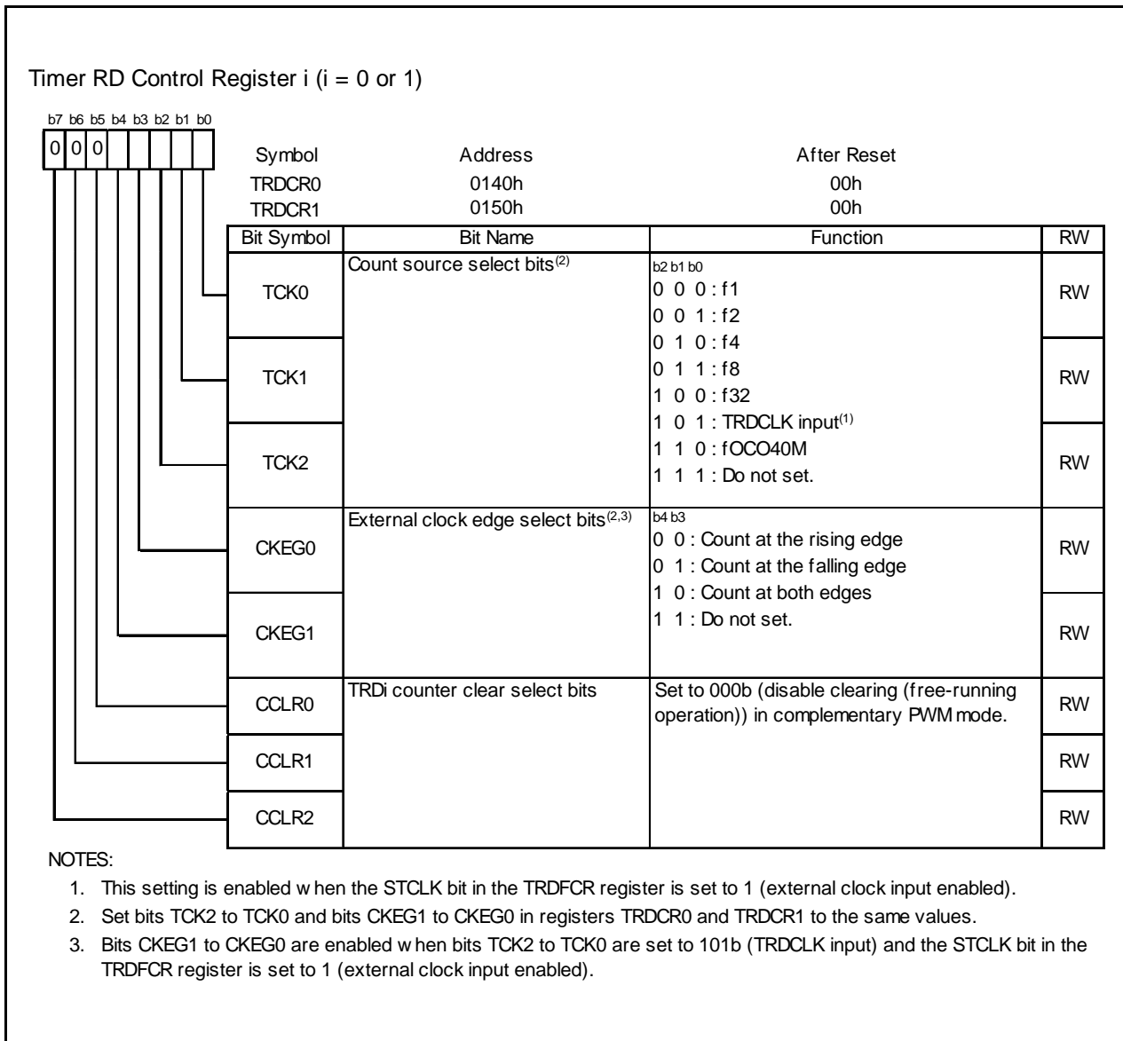
Figure 16.127 Registers TRDCR0 to TRDCR1 in Complementary PWM Mode
