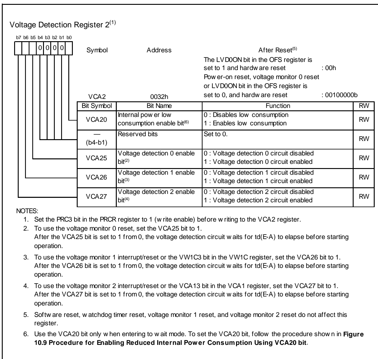
Figure 10.8 VCA2 Register
