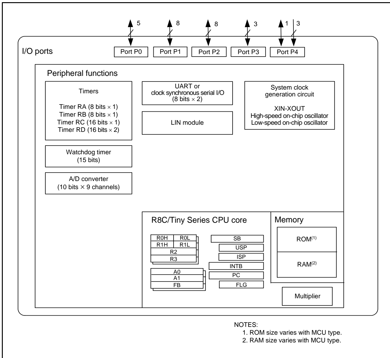
Figure 1.3 Block Diagram
