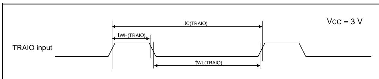
Figure 22.9 TRAIO Input Timing Diagram when V_{CC} = 3\text{ V}
