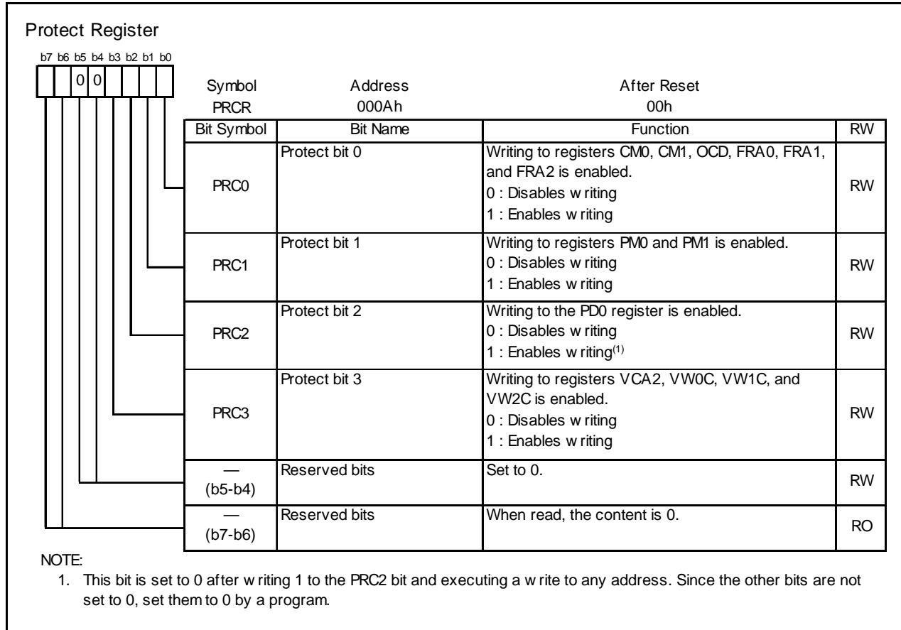
Figure 11.1 PRCR Register
