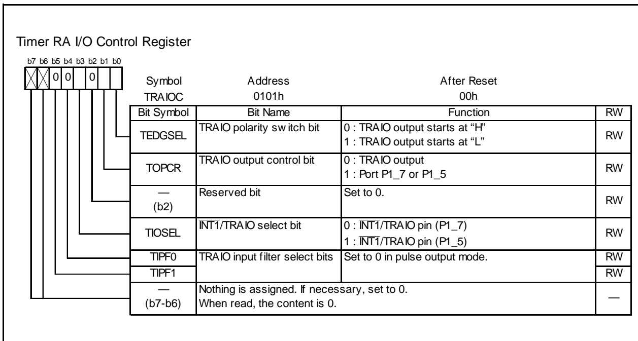
Figure 16.6 TRATIO Register in Pulse Output Mode
