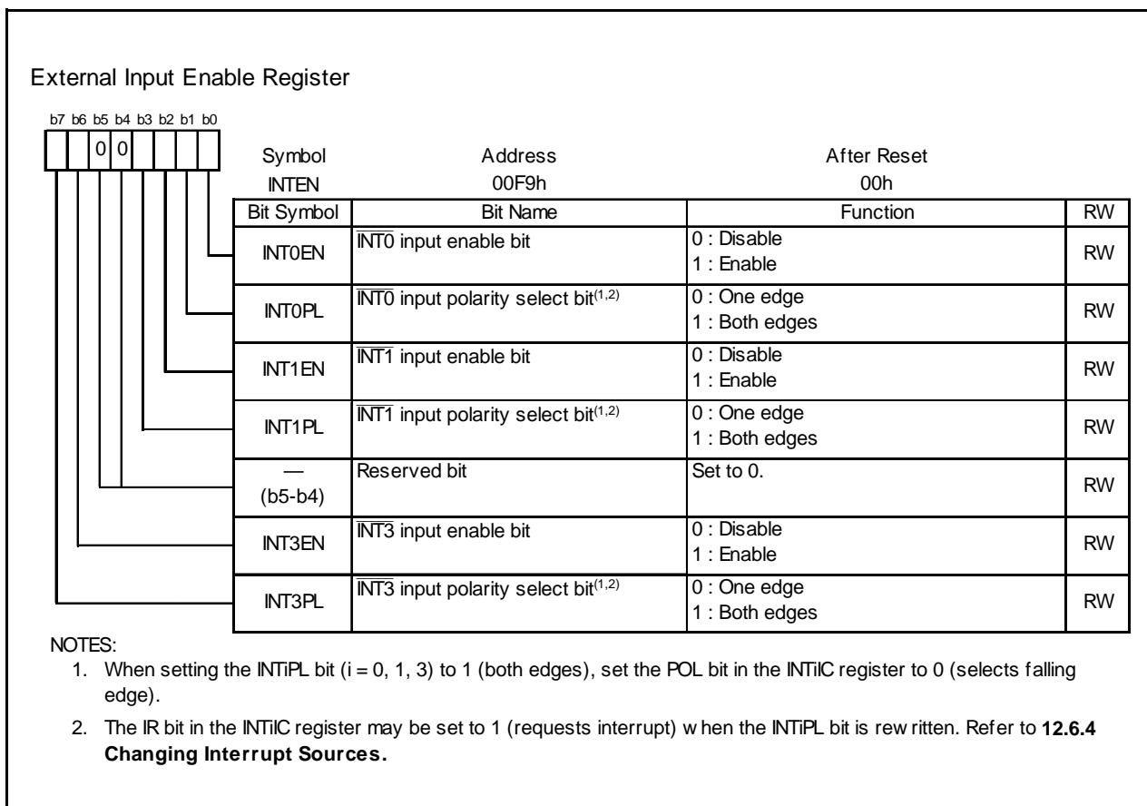
Figure 12.13 INTEN Register
