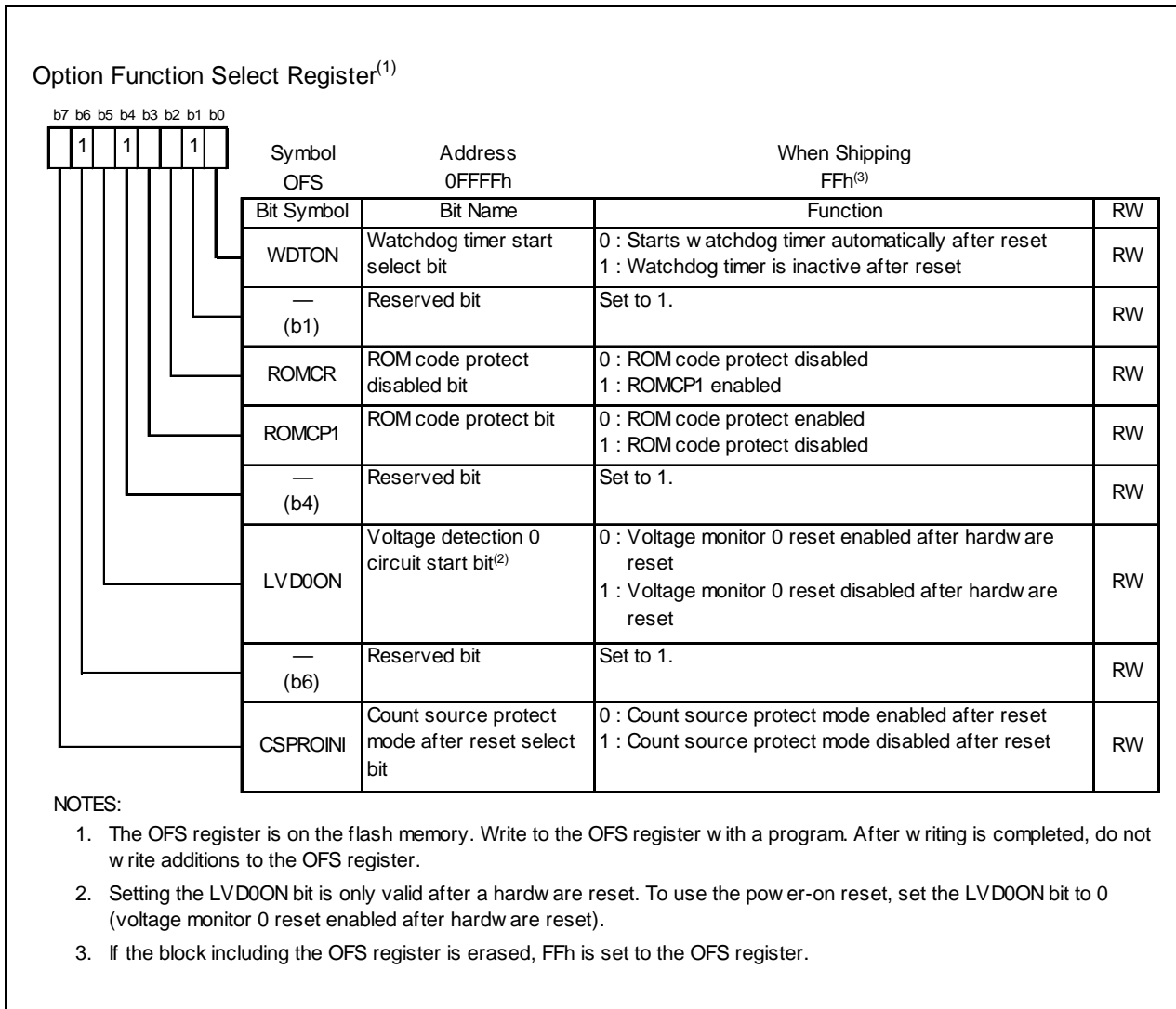
Figure 14.2 OFS Register
