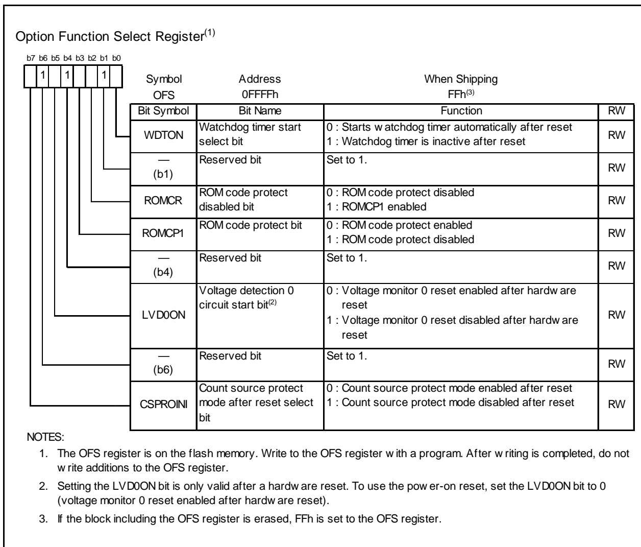
Figure 20.3 OFS Register
