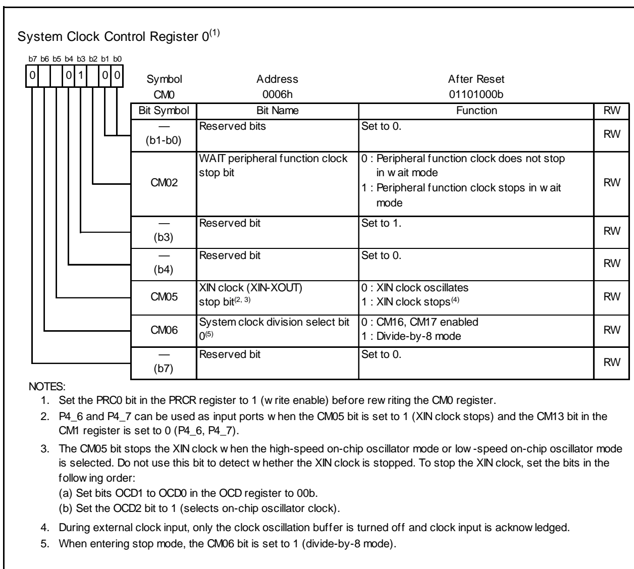
Figure 10.3 CM0 Register
