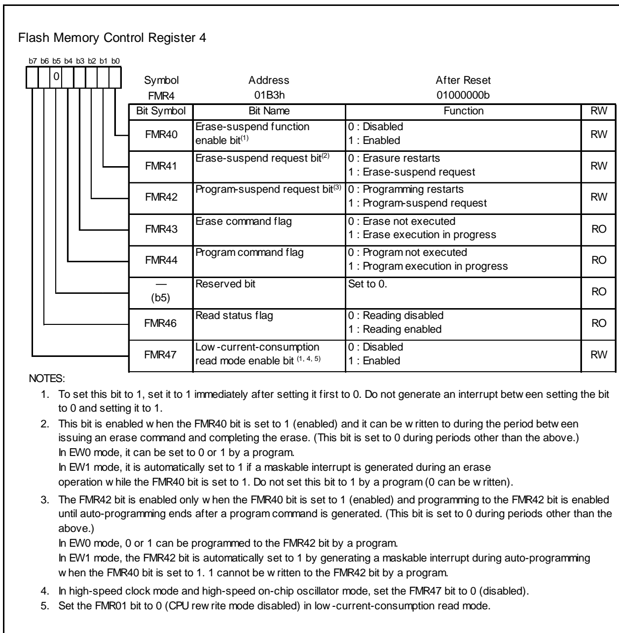
Figure 20.6 FMR4 Register
