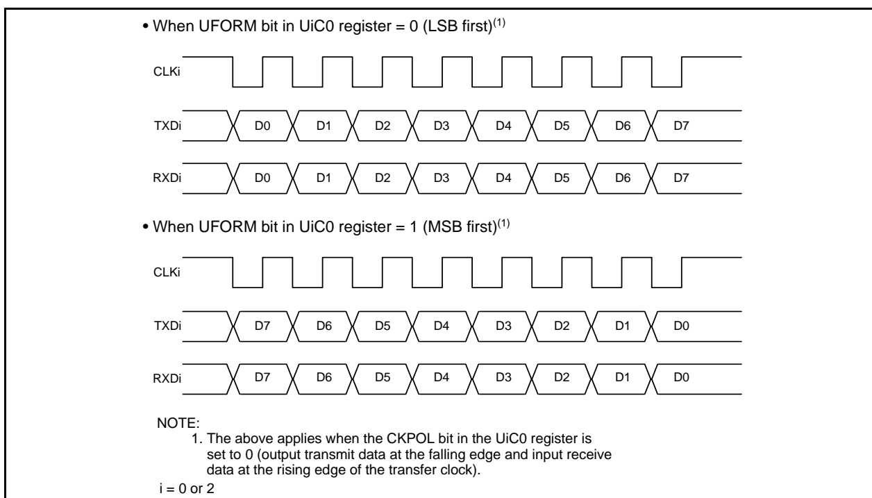
Figure 17.9 Transfer Format
