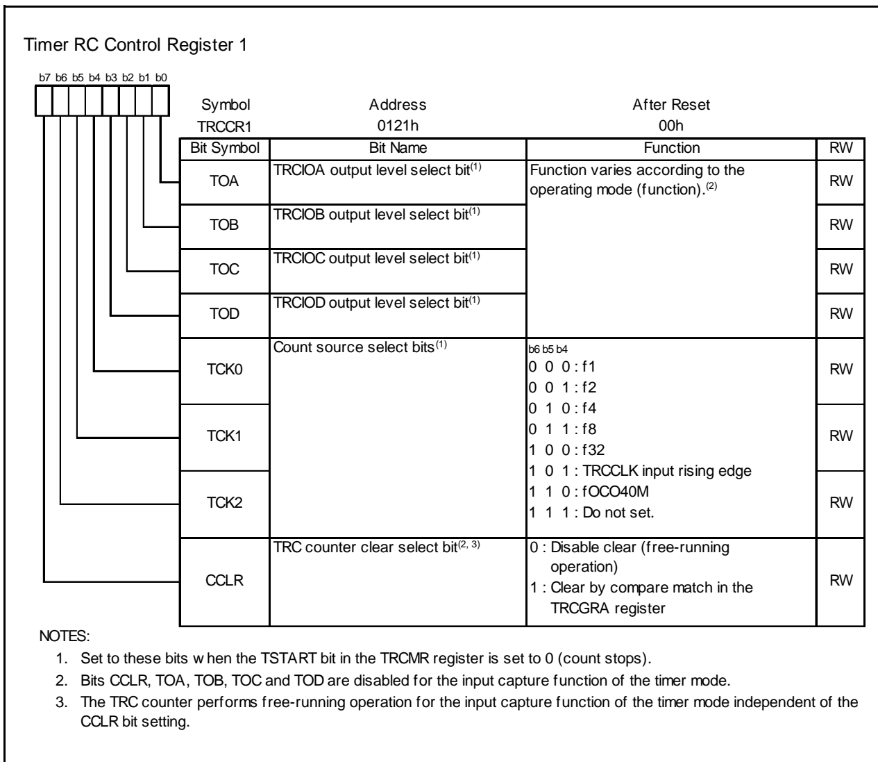
Figure 16.30 TRCCR1 Register
