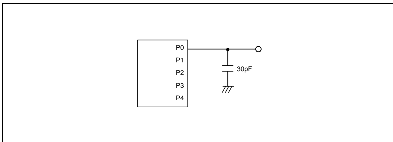
Figure 22.1 Ports P0 to P4 Timing Measurement Circuit
