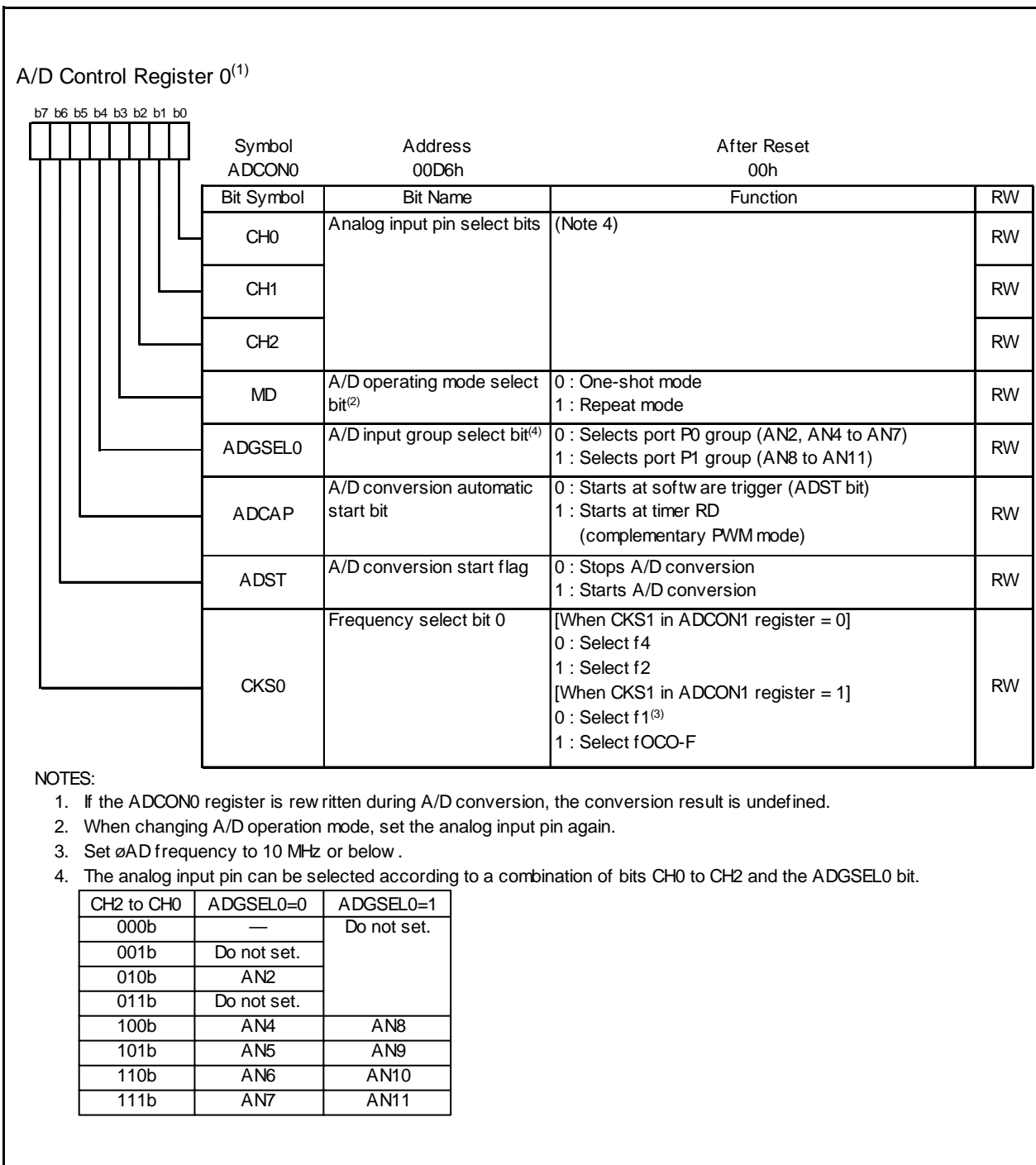
Figure 19.2 ADCON0 Register
