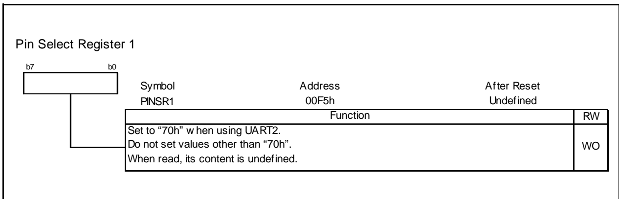
Figure 17.6 PINSR1 Register
