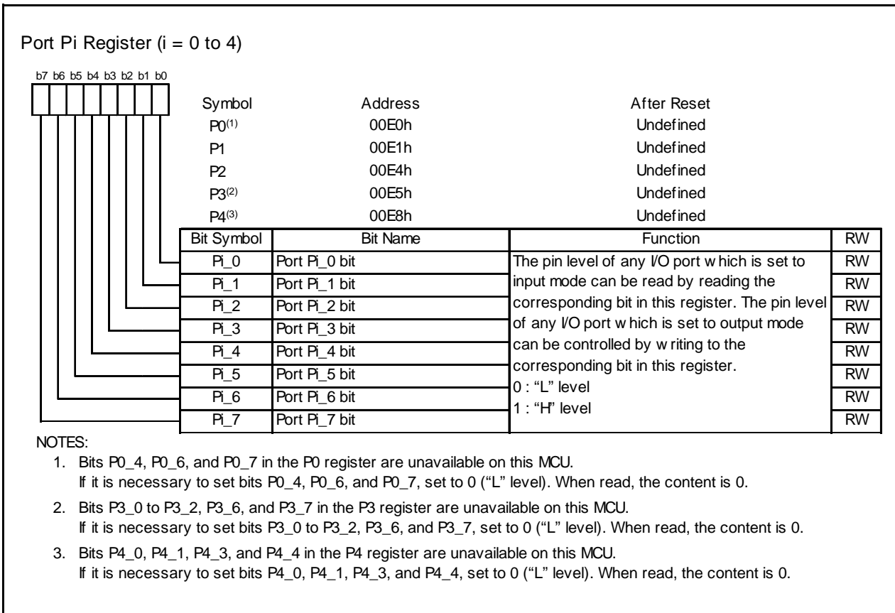
Figure 7.9 Pi (i = 0 to 4) Registers
