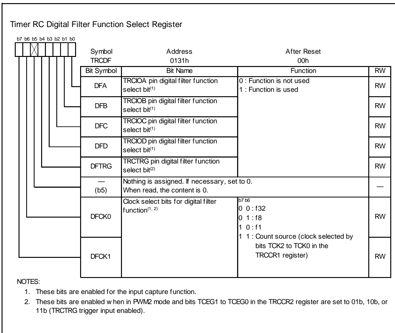
Figure 16.36 TRCDF Register
