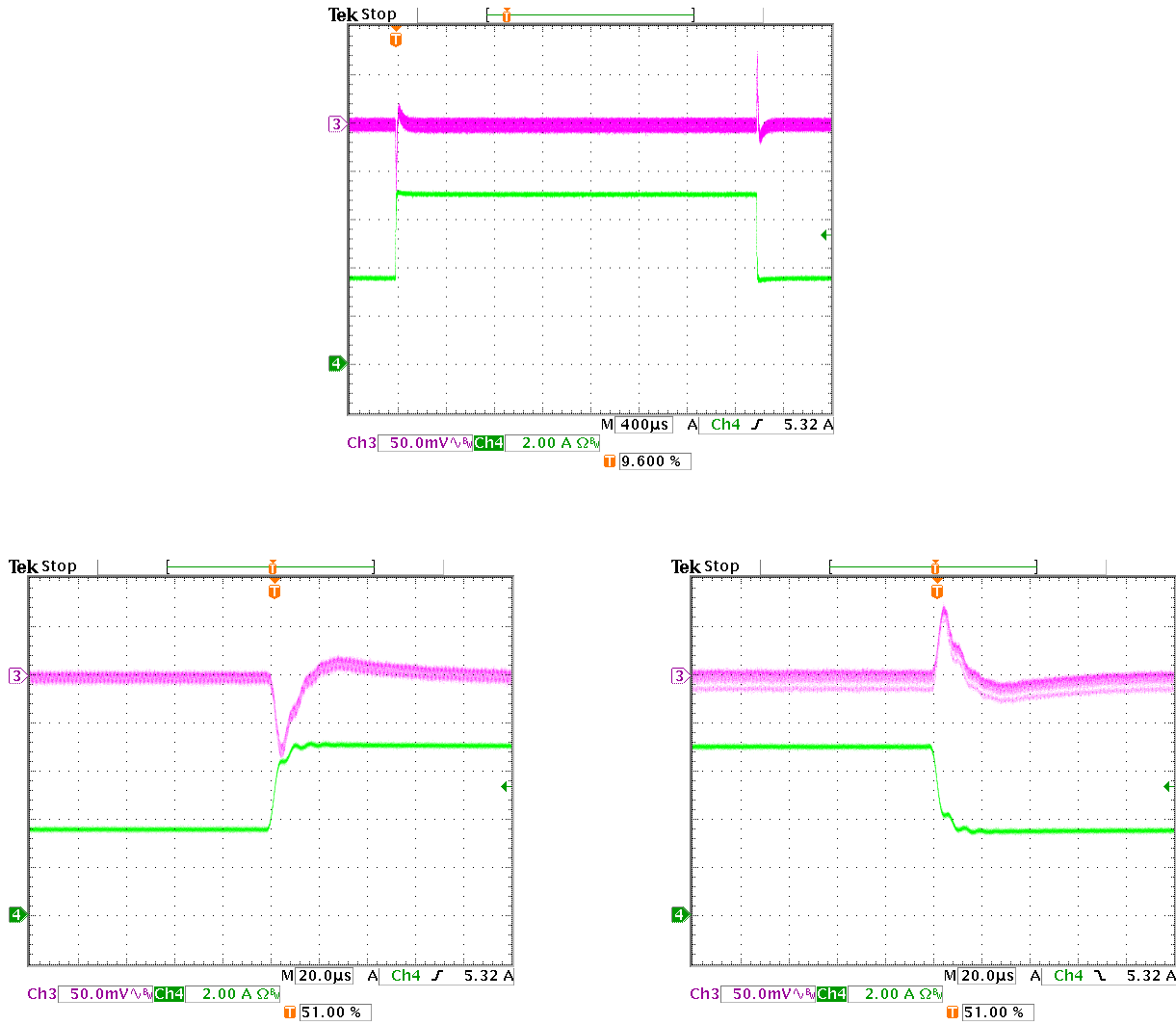
Fig. 13: Transient Response, 3.5A to 7A step Ch 3 :V out , Ch 4 :I out
