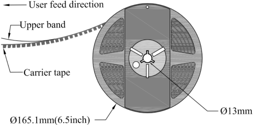
Figure 13. Reel dimensions for LUXEON 3030 HV.
