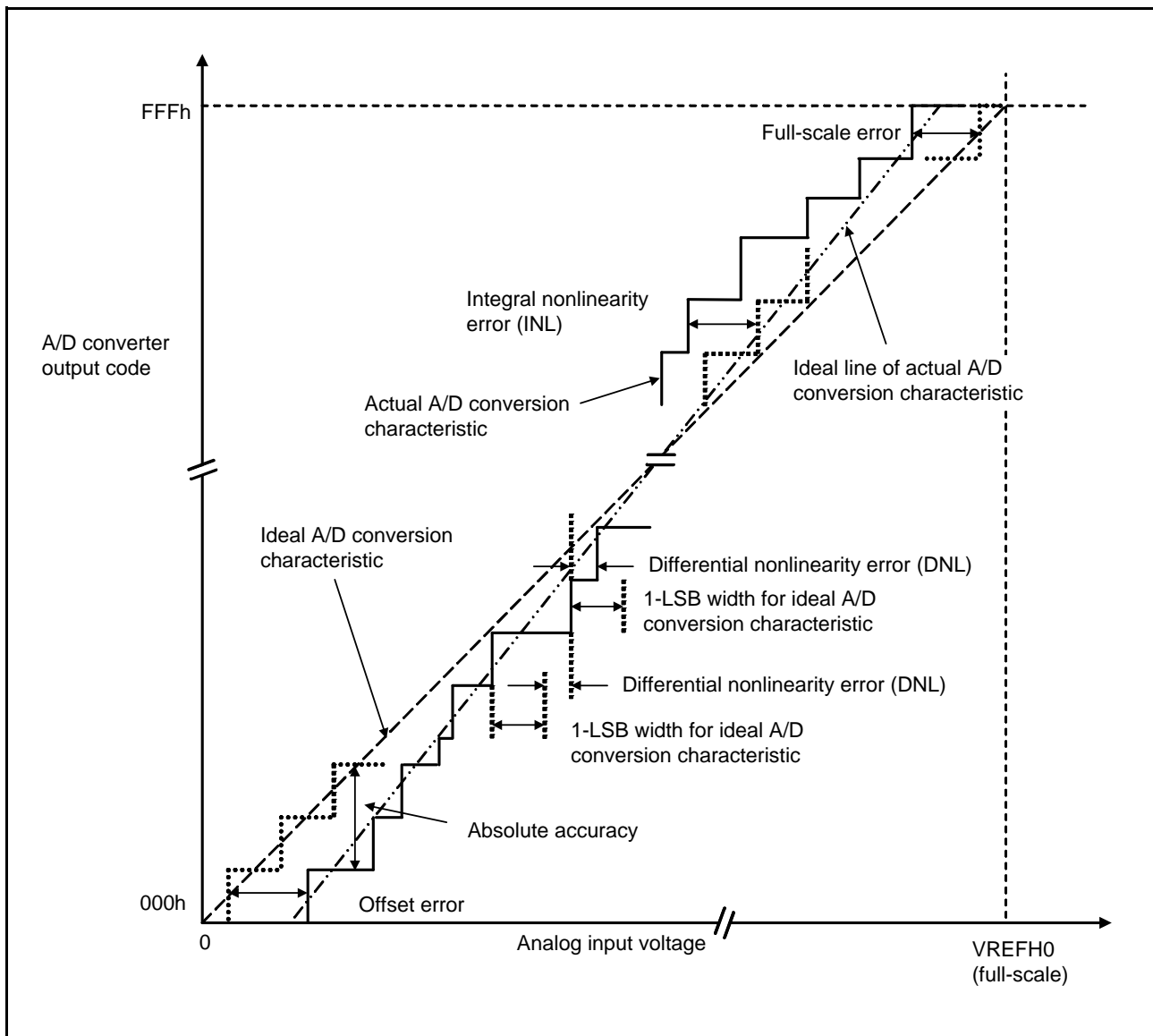
Figure 5.68 Illustration of A/D Converter Characteristic Terms
