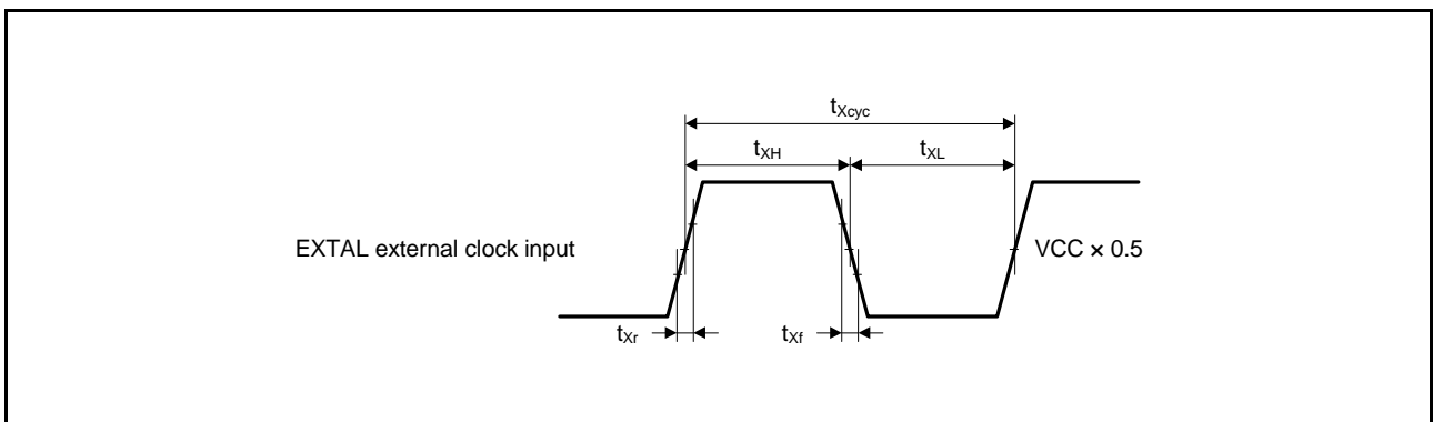
Figure 5.23 EXTAL External Clock Input Timing
