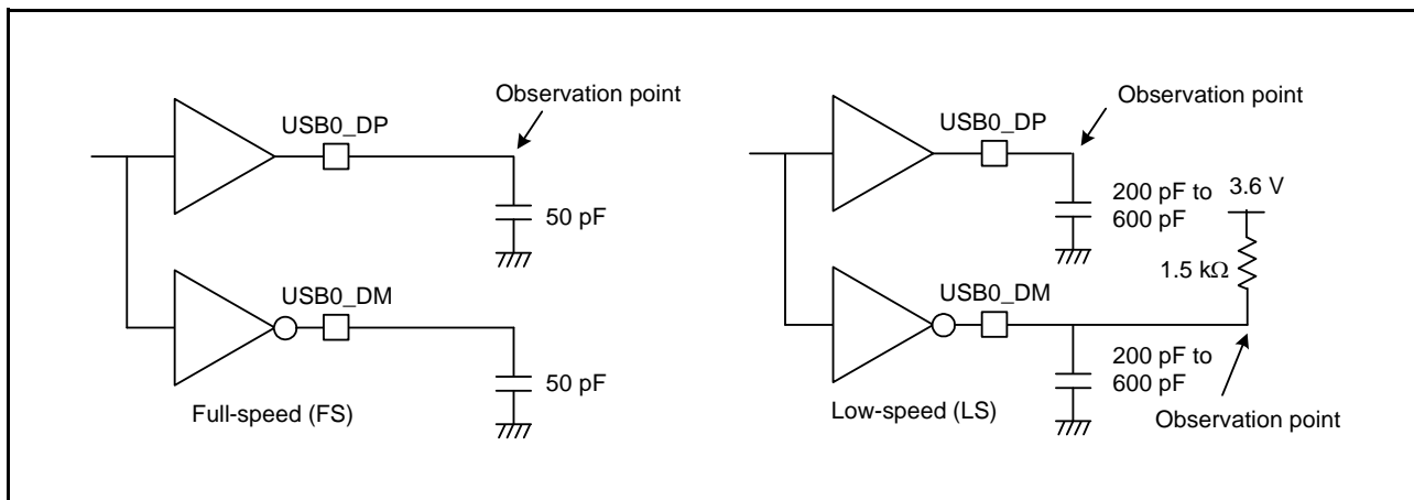
Figure 5.65 Test Circuit
