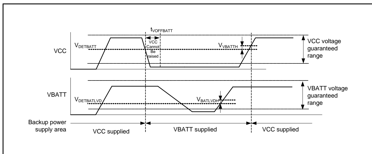
Figure 5.78 Battery Backup Function Characteristics
