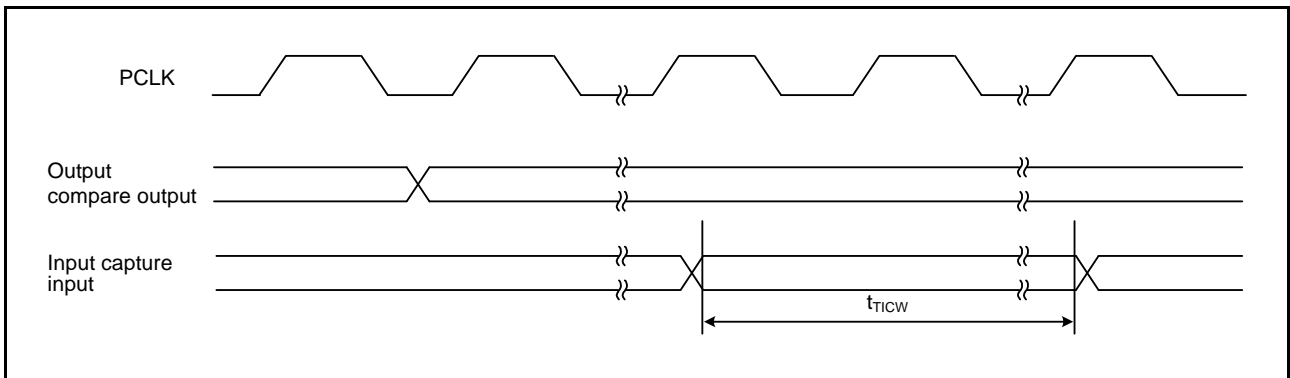
Figure 5.46 MTU2 Input/Output Timing
