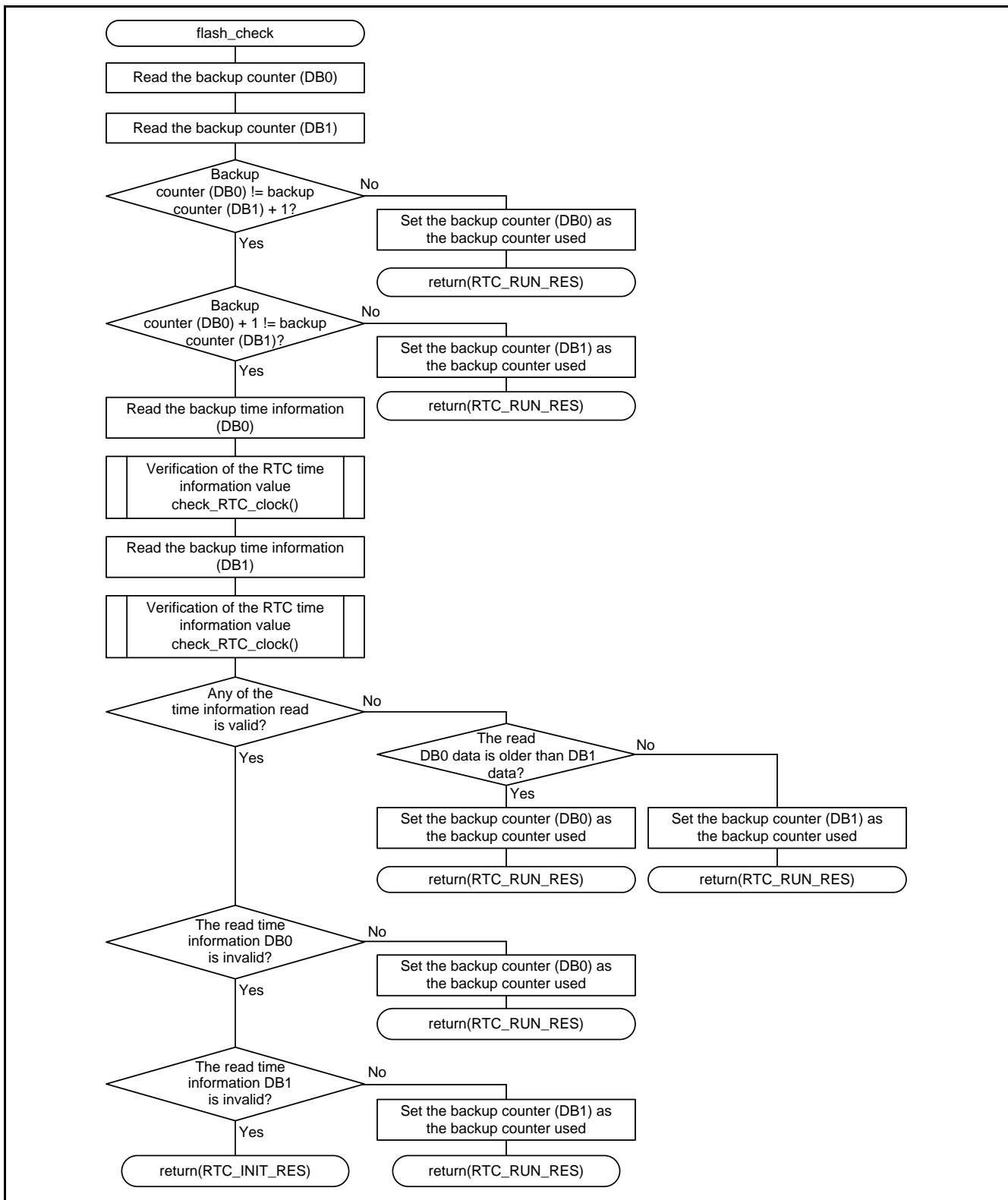
Figure 5.8 Determination of the Backup Time Information for Use
