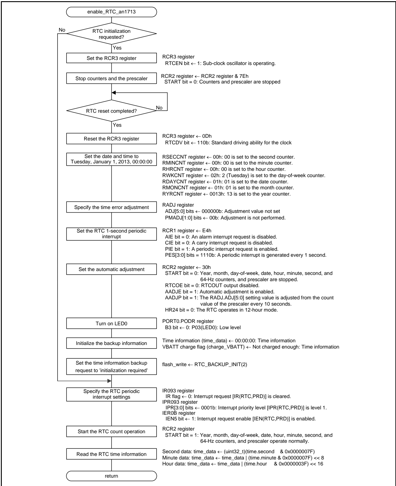
Figure 5.15 RTC Initialization
