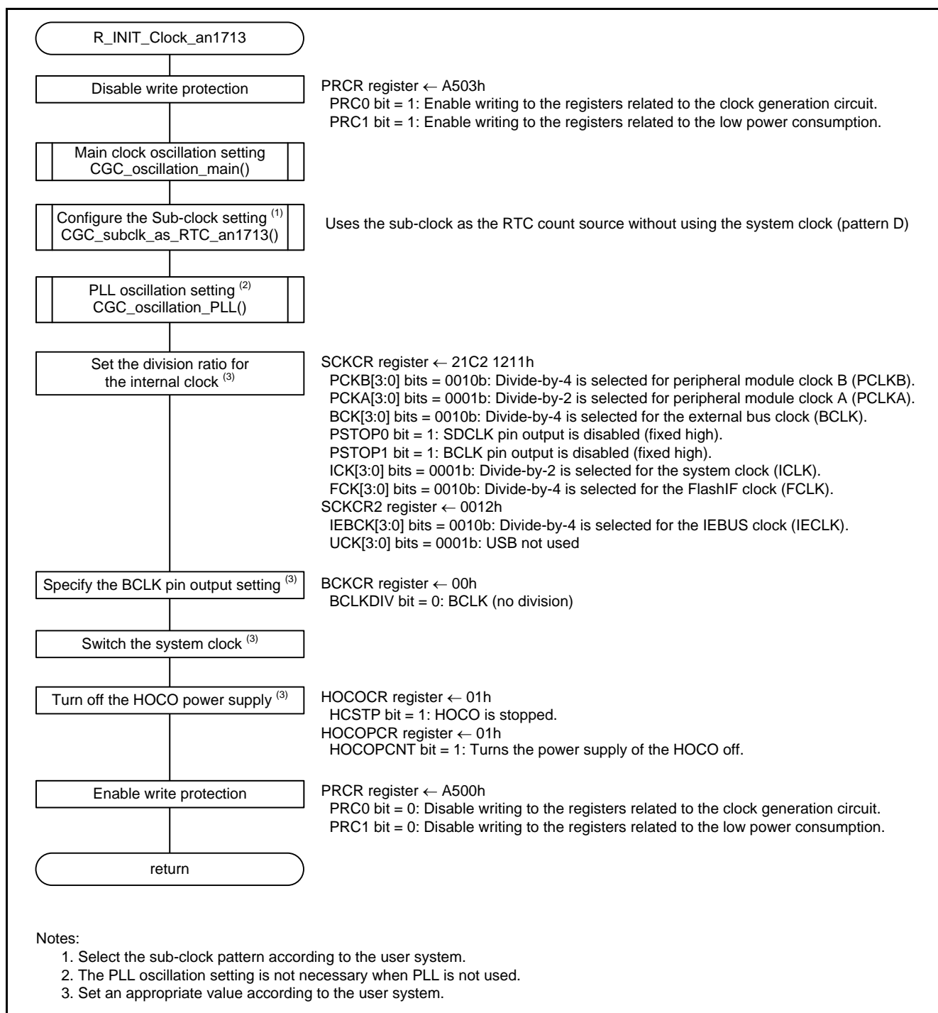
Figure 5.13 Clock Initialization
