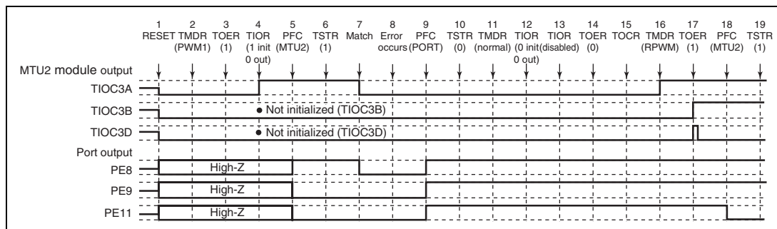
Figure 11.150 Error Occurrence in PWM Mode 1, Recovery in Reset-Synchronized PWM Mode
