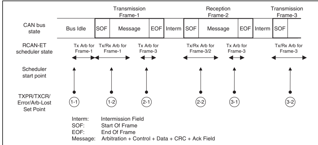
Figure 22.11 Internal Arbitration for Transmission
