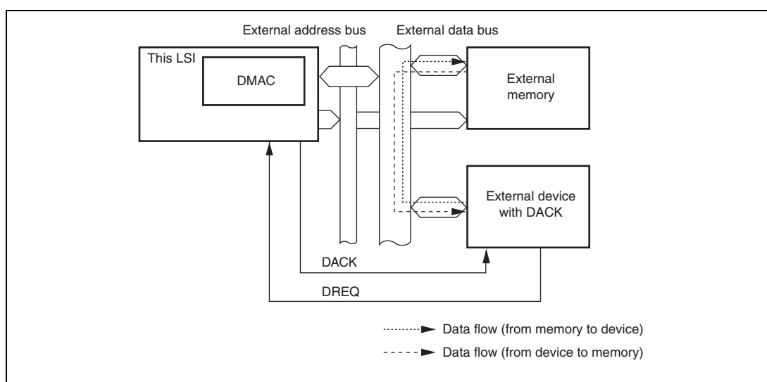
Figure 10.7 Data Flow in Single Address Mode
