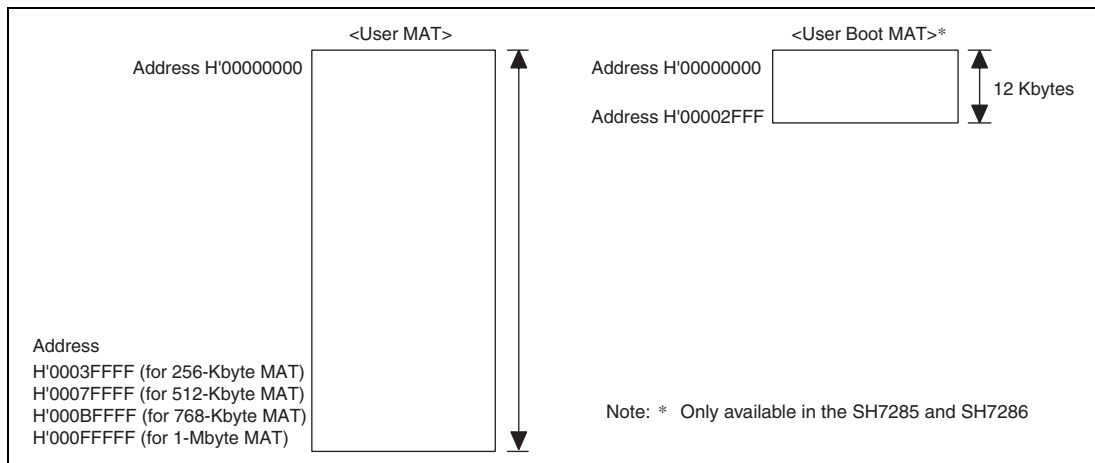
Figure 26.3 Flash Memory Configuration
