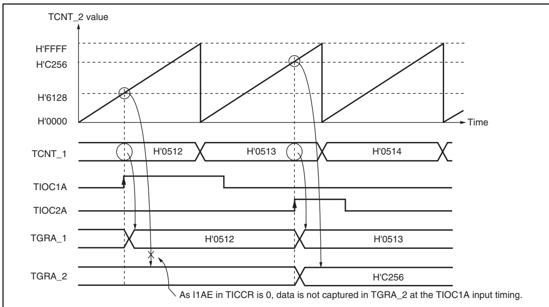
Figure 11.22 Cascaded Operation Example (b)
