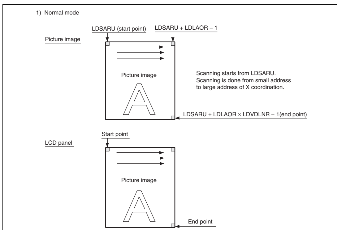
Figure 24.9 Operation for Hardware Rotation (Normal Mode)
