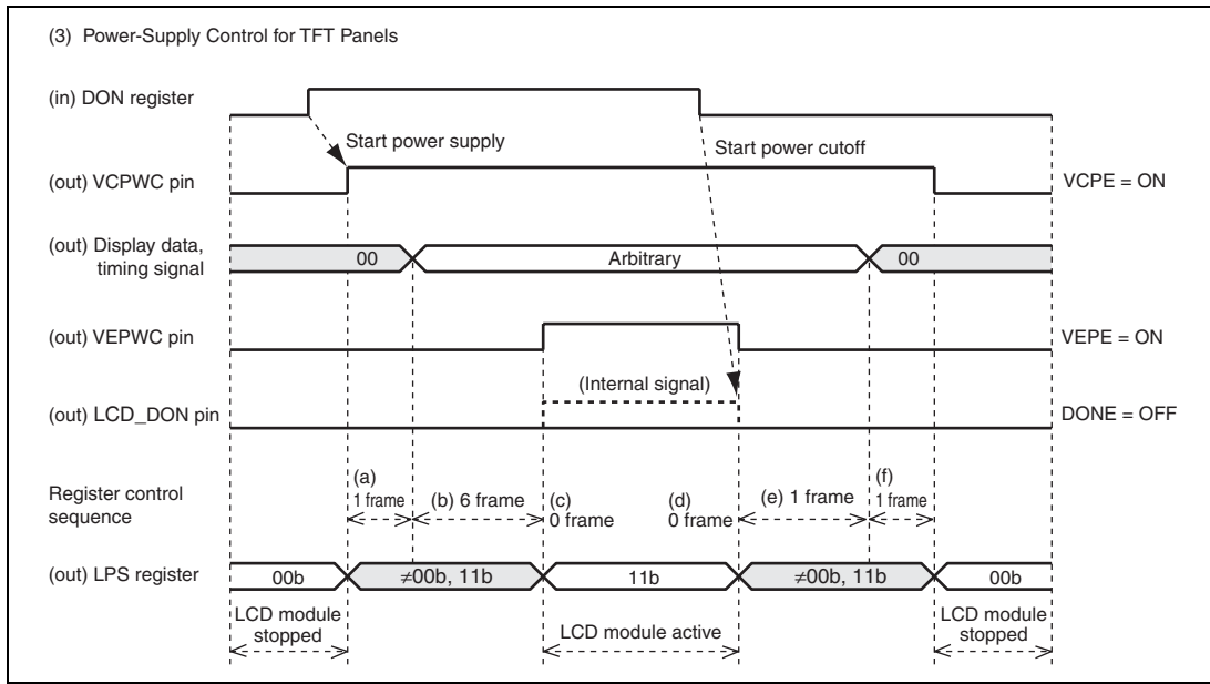
Figure 24.7 Power-Supply Control Sequence and States of the LCD Module
