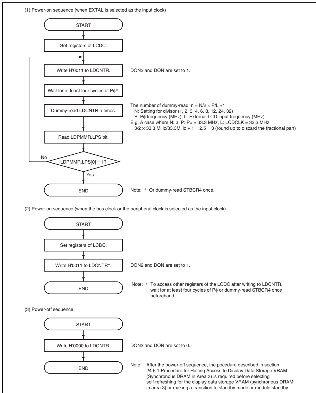
Figure 24.4 Flowchart for Power-Supply Control Sequence
