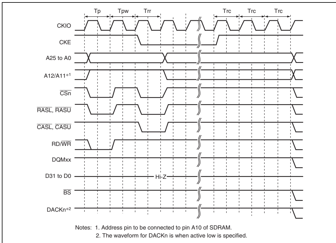
Figure 9.29 Self-Refresh Timing
