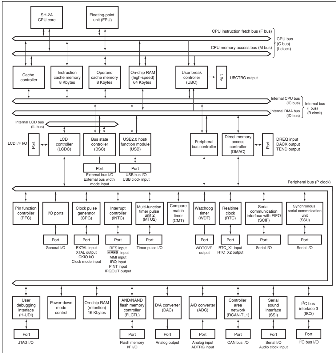
Figure 1.1 Block Diagram
