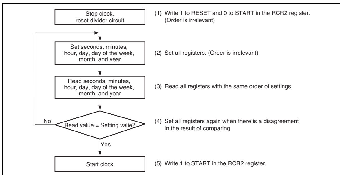
Figure 14.2 Setting Time
