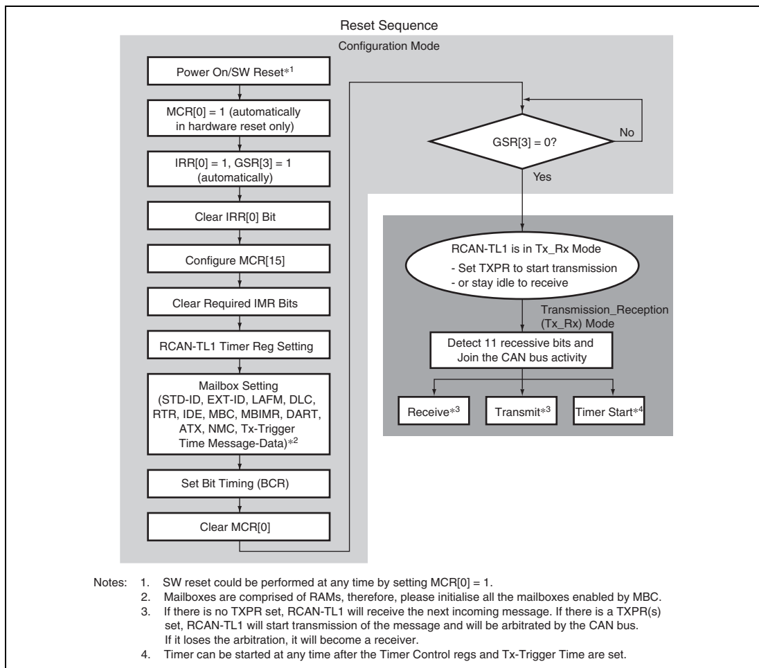
Figure 19.14 Reset Sequence
