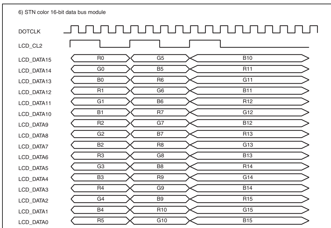
Figure 24.16 Clock and LCD Data Signal Example (STN Color 16-Bit Data Bus Module)
