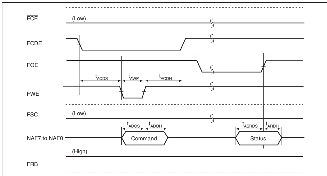
Figure 31.68 AND Type Flash Memory Status Read Timing
