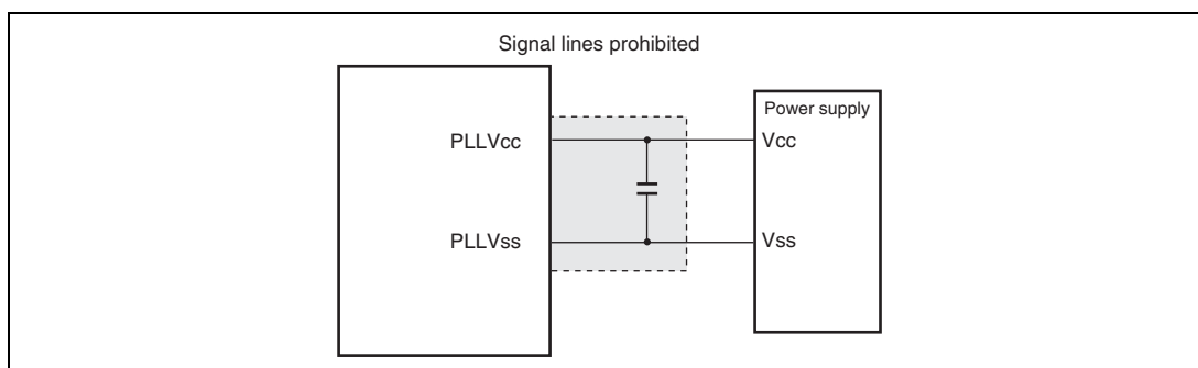
Figure 4.4 Note on Using a PLL Oscillation Circuit
