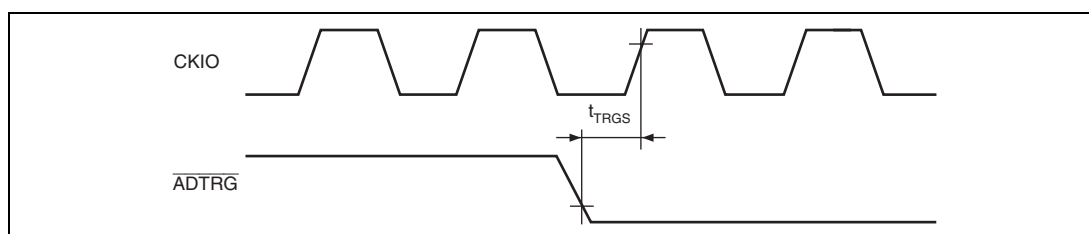
Figure 31.63 A/D Converter External Trigger Input Timing
