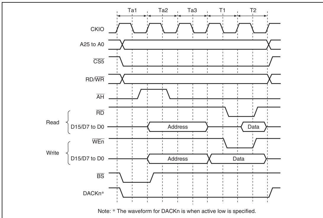
Figure 9.11 (1) Access Timing for MPX Space (Address Cycle No Wait, Data Cycle No Wait)
