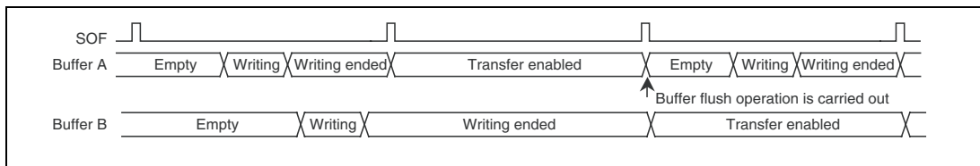
Figure 23.18 Example of Buffer Flush Function Operation
