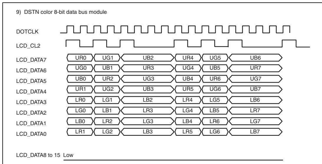
Figure 24.19 Clock and LCD Data Signal Example (DSTN Color 8-Bit Data Bus Module)
