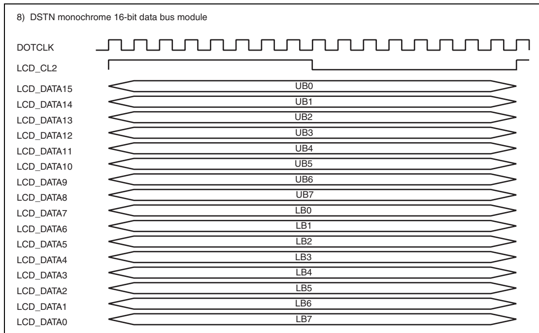
Figure 24.18 Clock and LCD Data Signal Example (DSTN Monochrome 16-Bit Data Bus Module)
