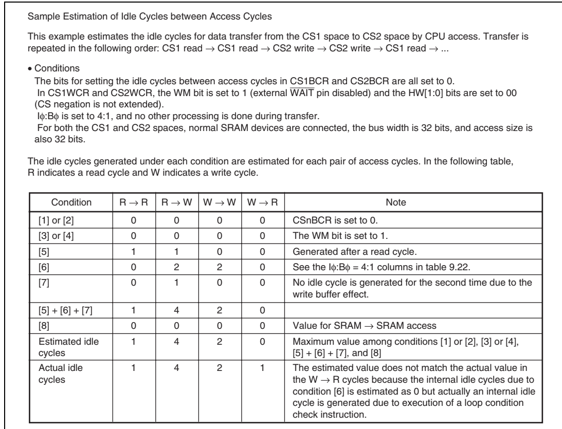
Figure 9.54 Comparison between Estimated Idle Cycles and Actual Value
