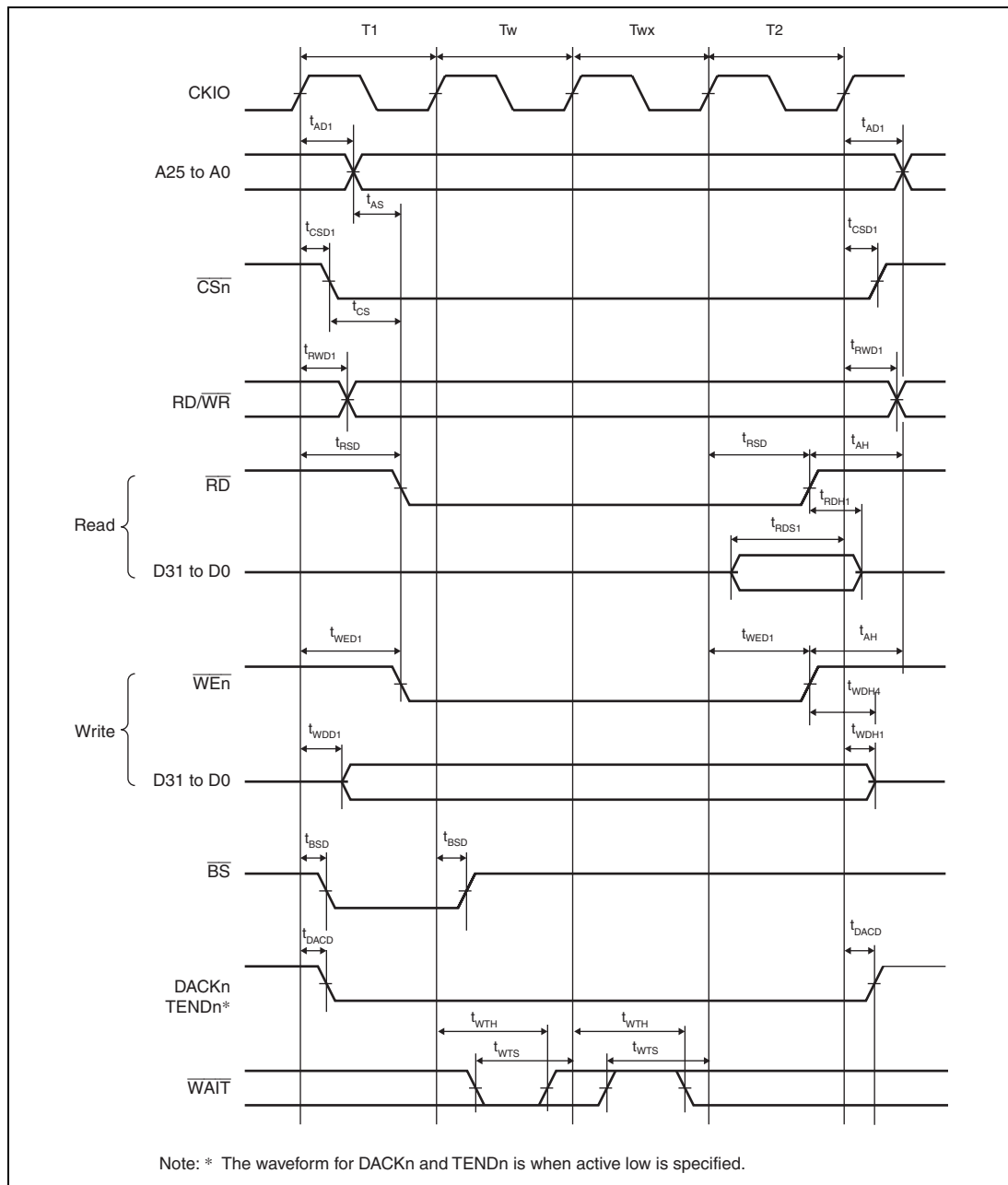
Figure 31.15 Basic Bus Timing for Normal Space (One Software Wait Cycle, One External Wait Cycle)
