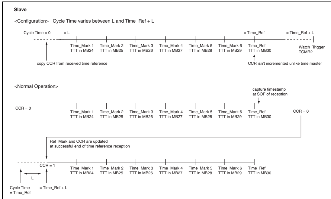
Figure 19.20 Time Slave
