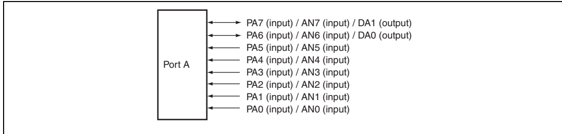
Figure 26.1 Port A
