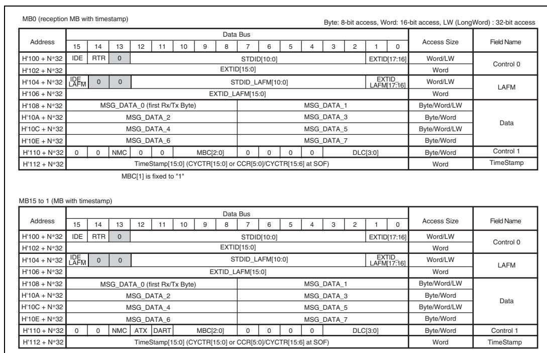
Figure 19.3 Mailbox-N Structure
