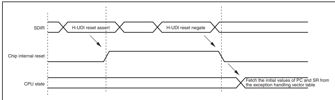
Figure 29.4 H-UDI Reset
