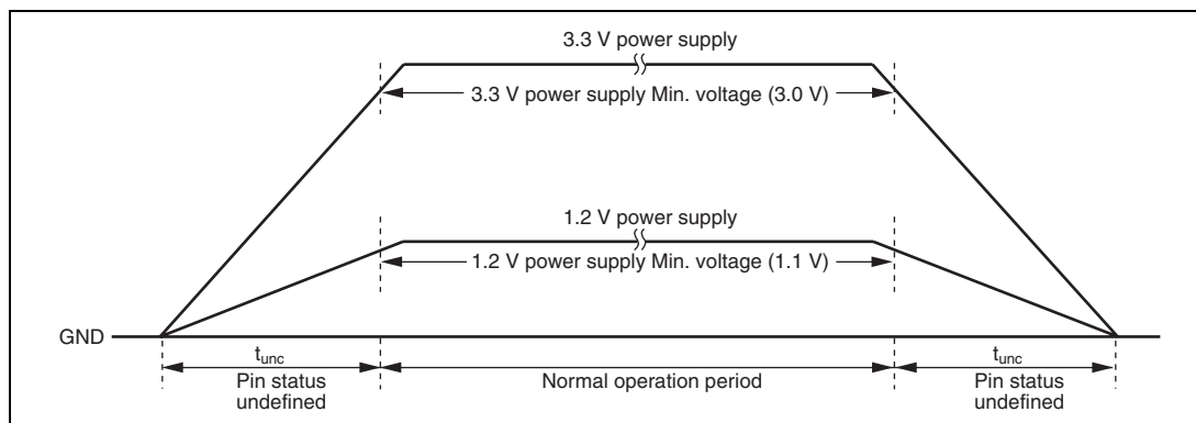
Figure 31.1 Power-on/Power-off Sequence
