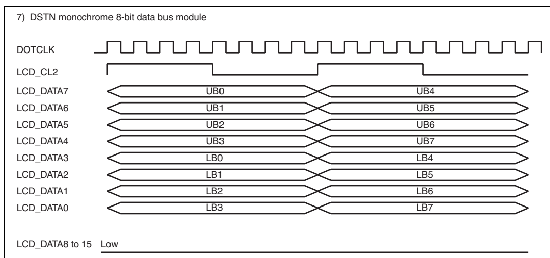
Figure 24.17 Clock and LCD Data Signal Example (DSTN Monochrome 8-Bit Data Bus Module)
