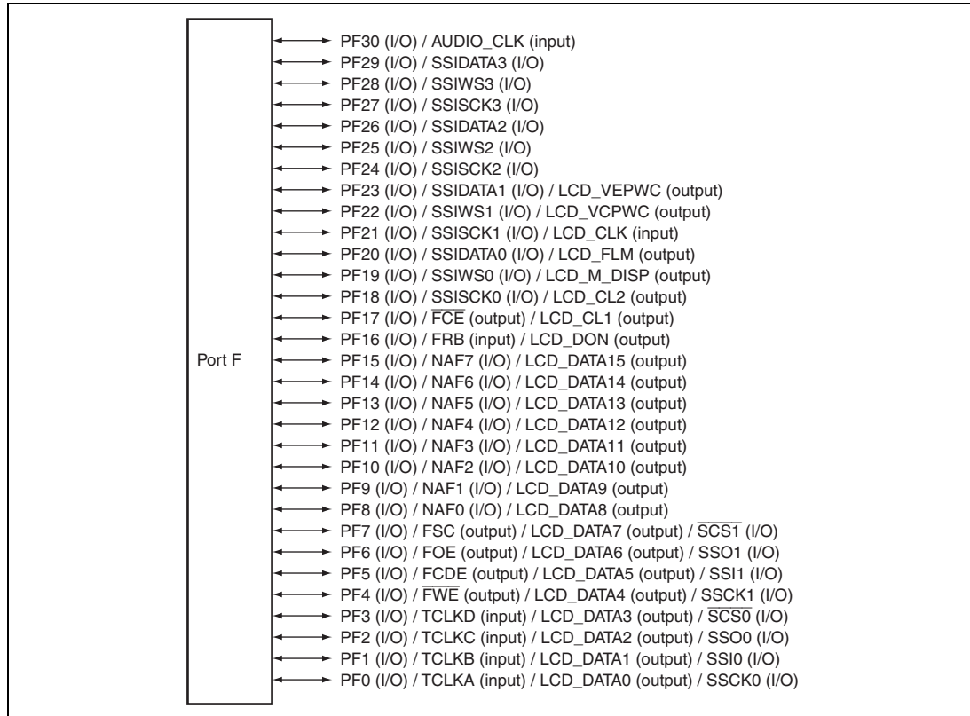
Figure 26.6 Port F
