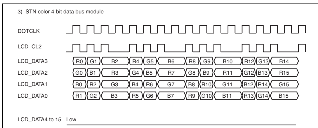
Figure 24.13 Clock and LCD Data Signal Example (STN Color 4-Bit Data Bus Module)
