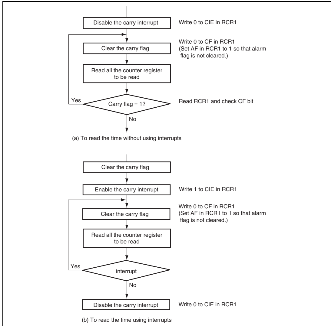
Figure 14.3 Reading Time
