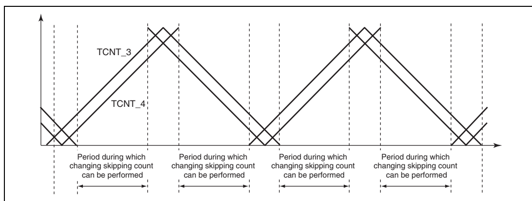
Figure 11.68 Periods during which Interrupt Skipping Count Can Be Changed
