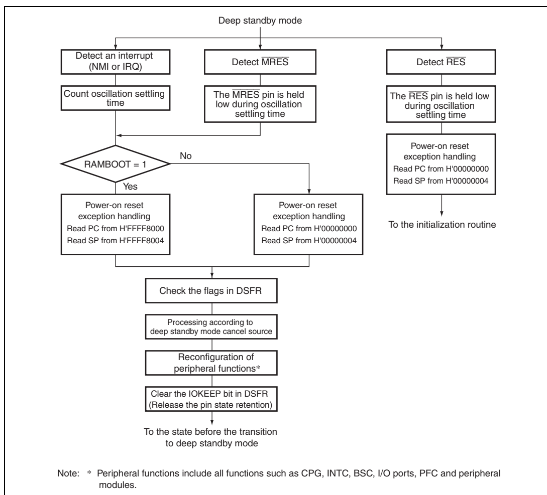
Figure 28.3 Flowchart of Canceling Deep Standby Mode
