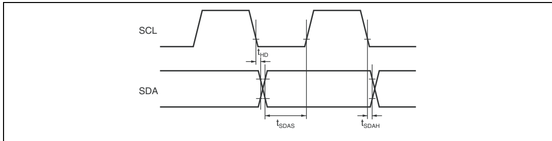
Figure 31.57 (3) Transmission and Reception Timing
