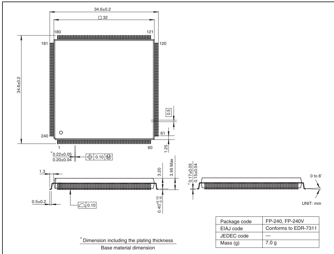
Figure C.1 Package Dimensions
