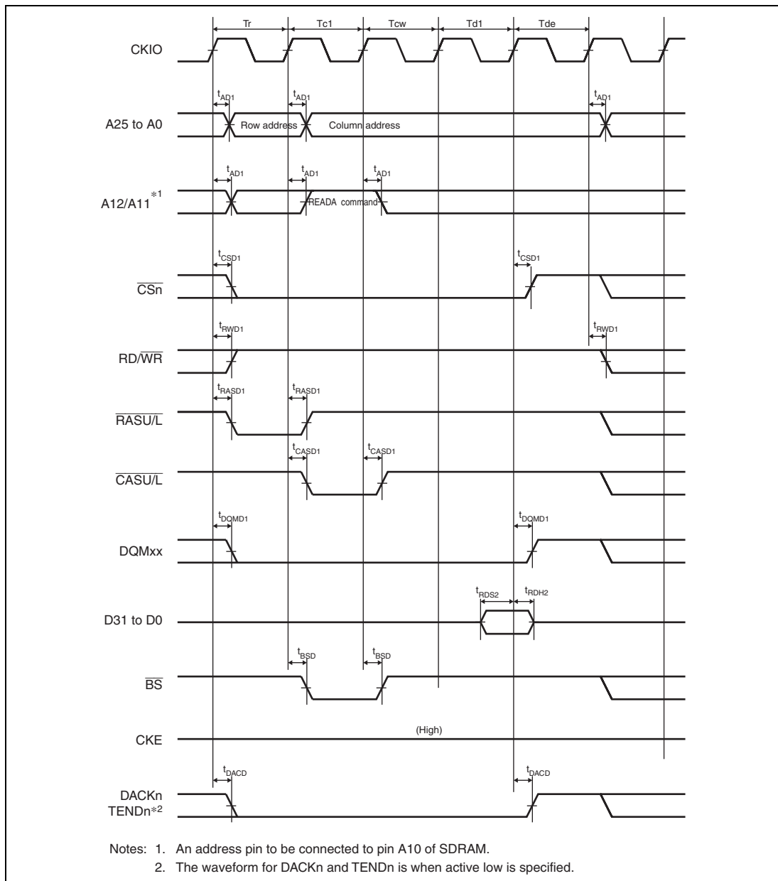
Figure 31.22 Synchronous DRAM Single Read Bus Cycle (Auto Precharge, CAS Latency 2, WTRCD = 0 Cycle, WTRP = 0 Cycle)
