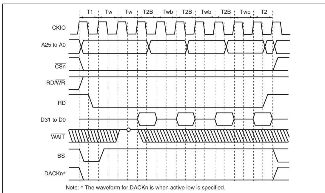
Figure 9.35 Burst ROM Access Timing (Clocked Asynchronous) (Bus Width = 32 Bits, 16-Byte Transfer (Number of Burst 4), Wait Cycles Inserted in First Access = 2, Wait Cycles Inserted in Second and Subsequent Access Cycles = 1)
