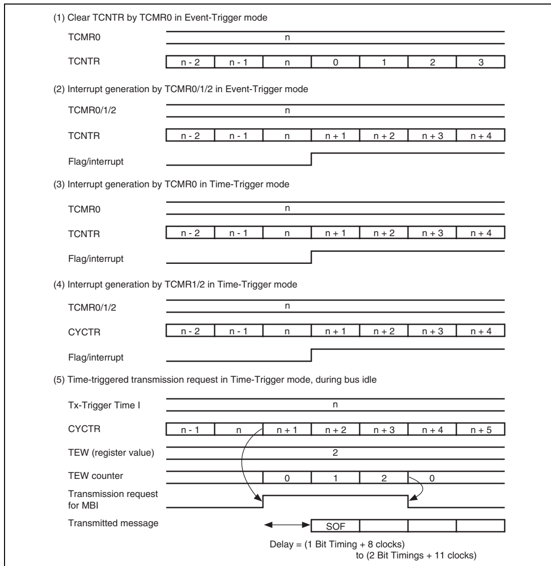
Figure 19.23 Timing Diagram of Timer
