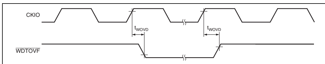
Figure 31.50 WDT Timing
