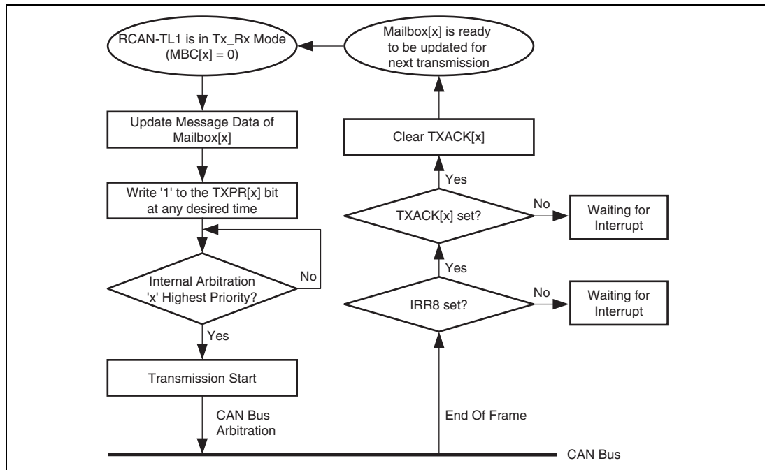
Figure 19.16 Transmission request
