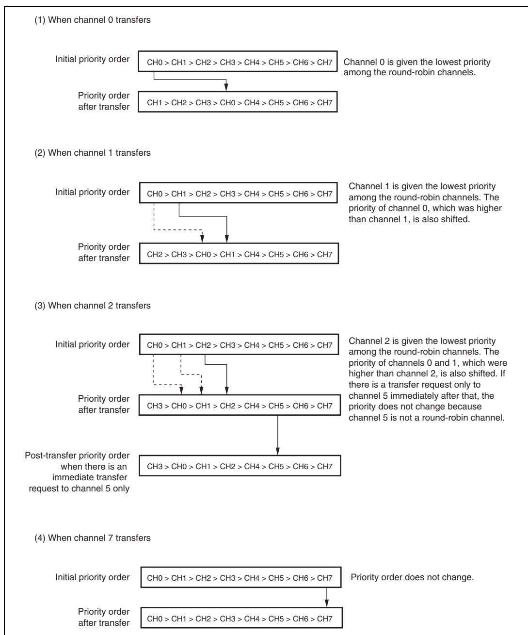
Figure 10.3 Round-Robin Mode
