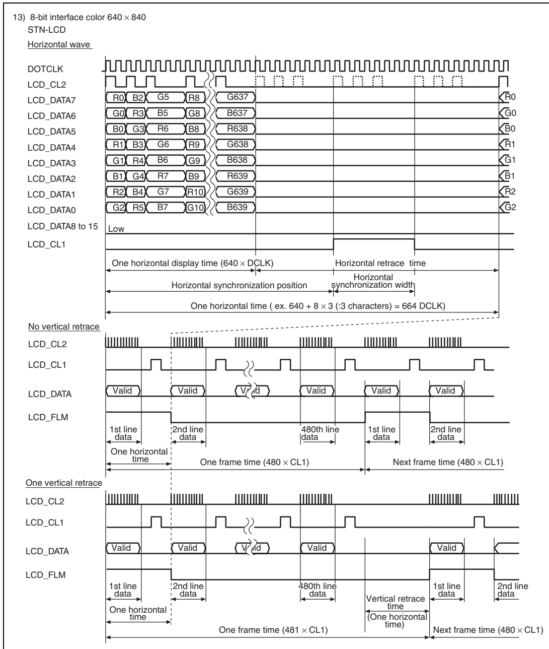
Figure 24.23 Clock and LCD Data Signal Example (8-Bit Interface Color 640 × 480)
