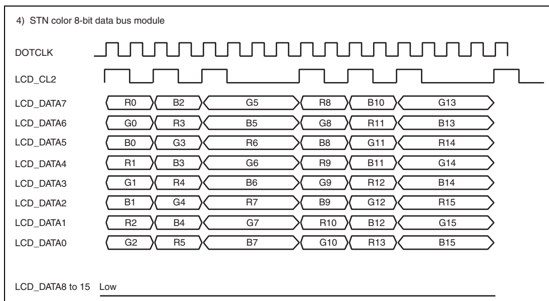
Figure 24.14 Clock and LCD Data Signal Example (STN Color 8-Bit Data Bus Module)
