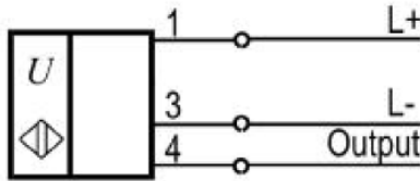
3RG6013-3AD00-PF:
