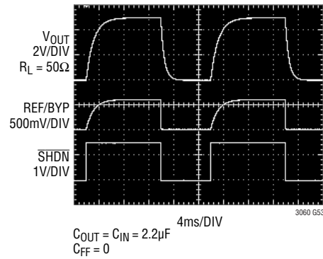
SHDN Transient Response C_{REF/BYP} = 10\text{nF}
