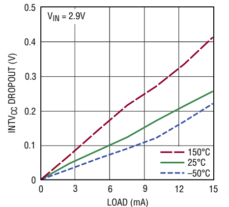
INTV CC Dropout vs Load and Temperature
