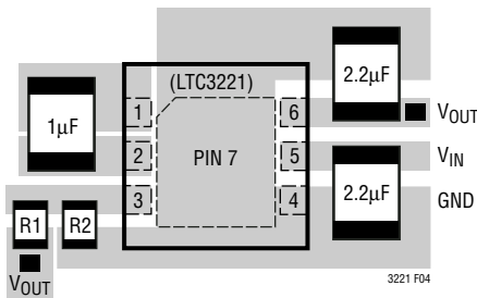
Figure 4. Recommended Layout
