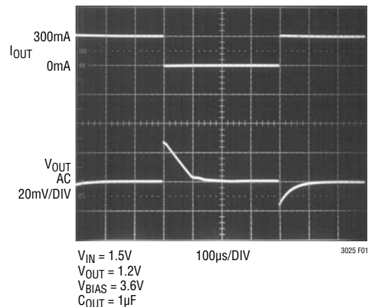
Figure 1. LTC3025 Transient Response
