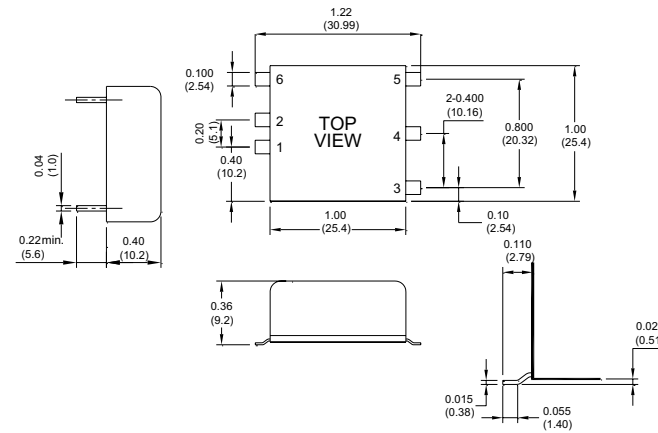
SMD- PACKAGE
