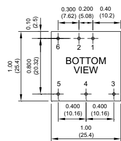
THROUGH-HOLE PACKAGE
