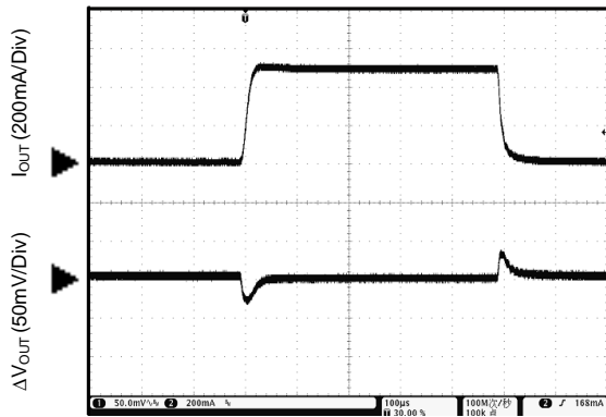
Load Transient Response (Conditions: V_{IN} = 2.5V, V_{OUT} = 1.25V, I_{OUT} = 1 \text{ to } 500mA ) C_{IN} = 1\mu F, C_{OUT} = 2.2\mu F
