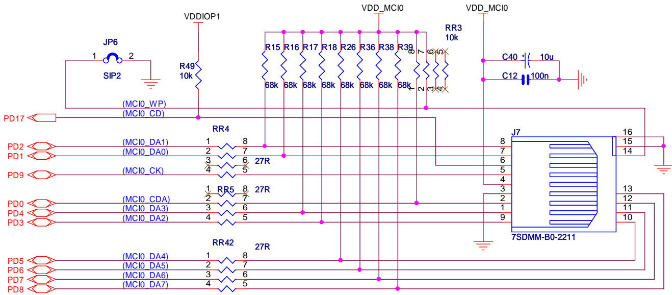
SD/MMCPlus CARD INTERFACE - MCIO
