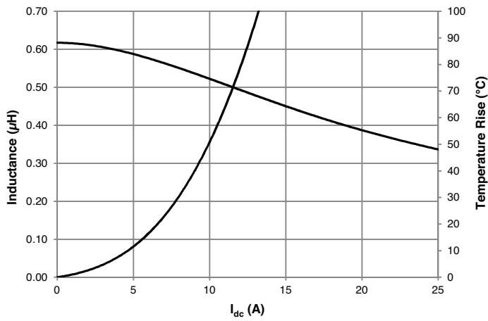
HCM1A0503-R68-R
