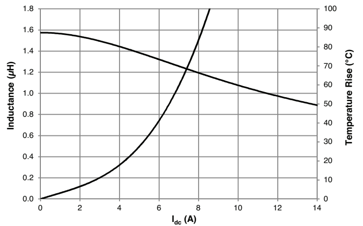
HCM1A0503-1R5-R
