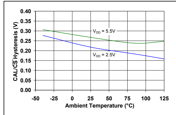
FIGURE 2-47: \text{CAL}/\overline{\text{CS}} Hysteresis vs. Ambient Temperature.
