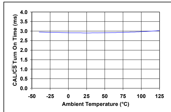
FIGURE 2-48: \text{CAL}/\overline{\text{CS}} Turn On Time vs. Ambient Temperature.
