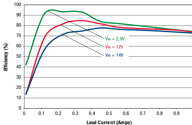
Efficiency vs. Line Voltage and Load Current @Ta = +25 °C (Vout = 1.5V)
