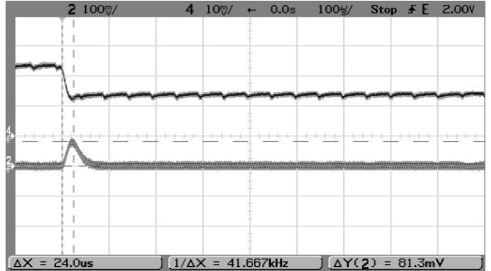
Step Load Transient Response (Vin=14V, Vout=2.5V, Cload=0, Iout=1A to 0.5A, Ta=+25°C.) Trace 2=Vout, 100 mV/div. Trace 4=Iout, 0.5A/div.
