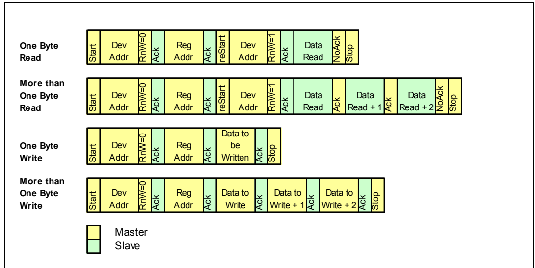
Figure 3. Operating modes
