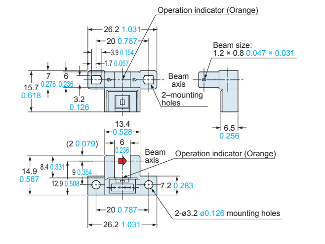
PM-F65 PM-F65-P Sensor
