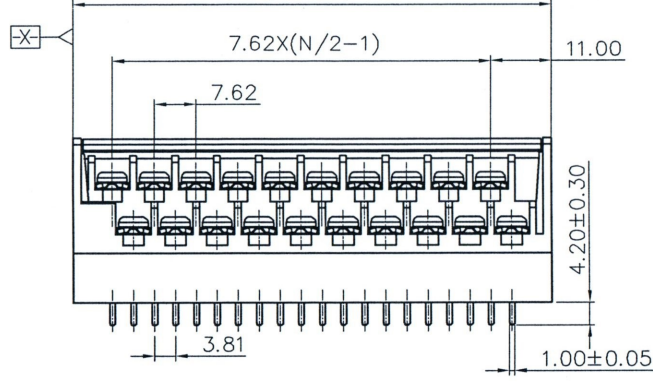
SEC B-B(PART) 7.62X(N/2-1)+18.18
