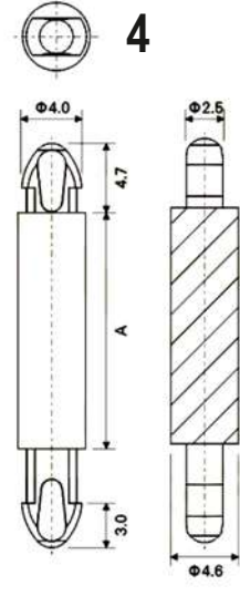
Top & Bottom Hole \varnothing 3.5 \pm 0.05 mm Top Panel Thickness 1.57 mm Bottom Panel Thickness 3.6 mm Type 4
