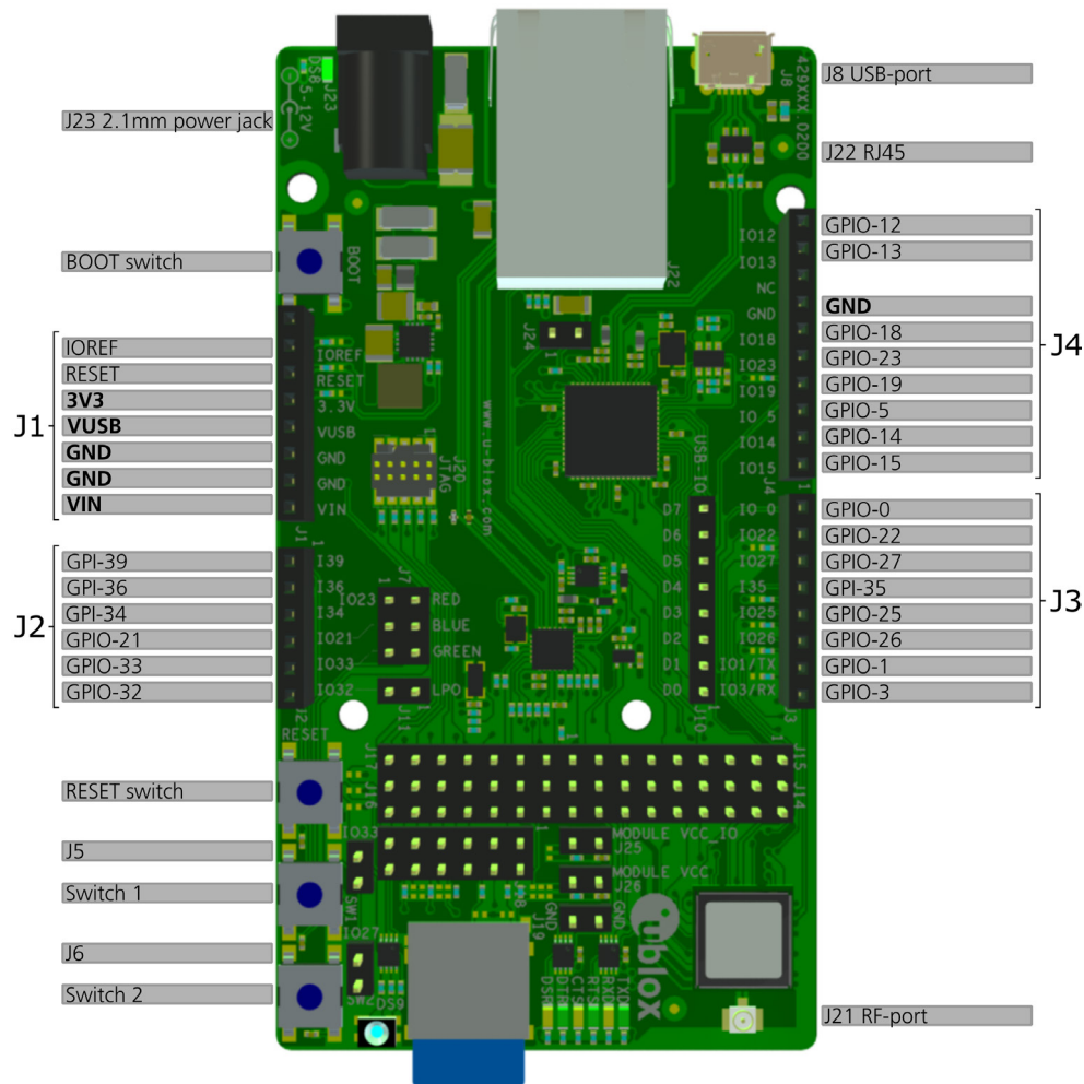
Figure 7: EVK-NINA-W13 connectors
