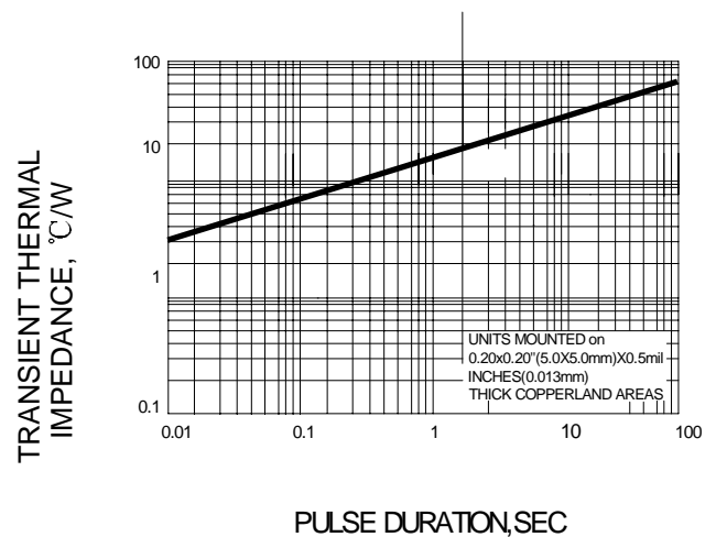
FIG.6-TRANSIENT THERMAL IMPEDANCE
