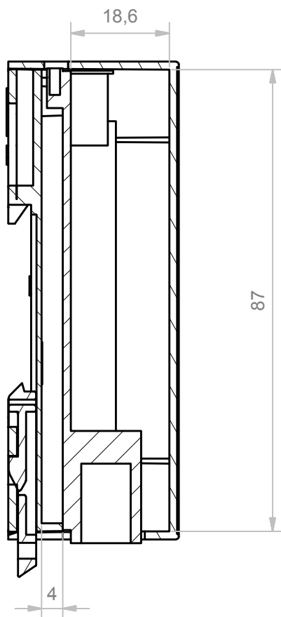
B-B (1:1)
