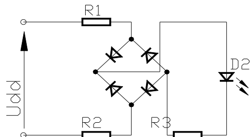
Full-wave rectifier
