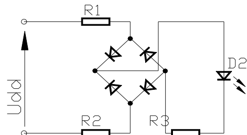
Full-wave rectifier
