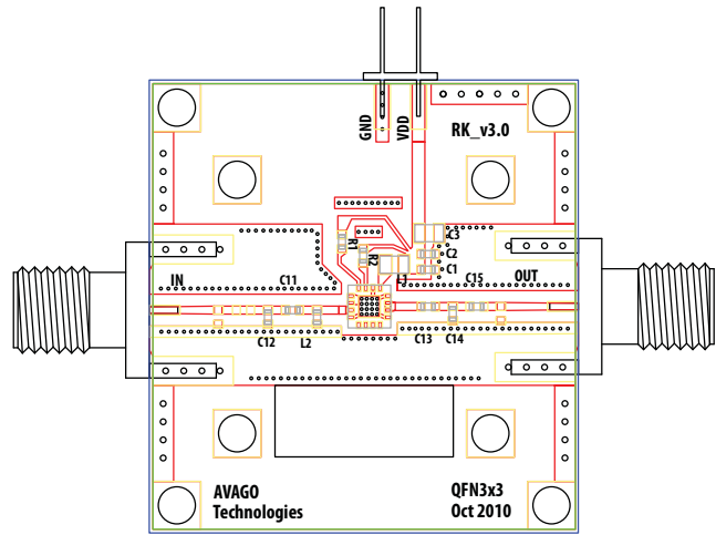
Figure 47. Demoboard
