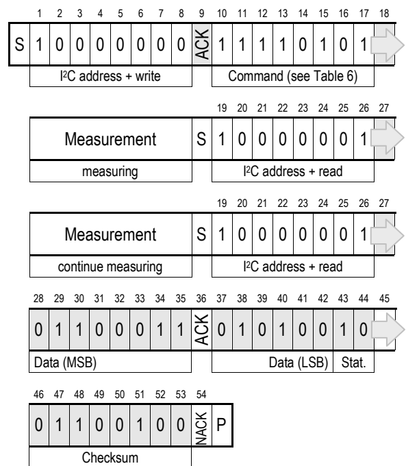
Figure 16 No Hold master communication sequence – grey blocks are controlled by SHT2x. If measurement is not completed upon “read” command, sensor does not provide ACK on bit 27 (more of these iterations are possible). If bit 45 is changed to NACK followed by Stop condition (P) checksum transmission is omitted.
