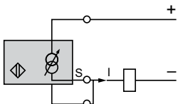
2-wire connection
