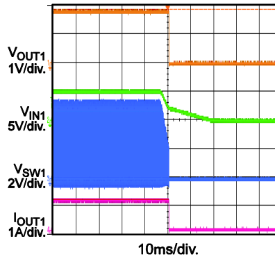
V IN Power Down with 1A Load
