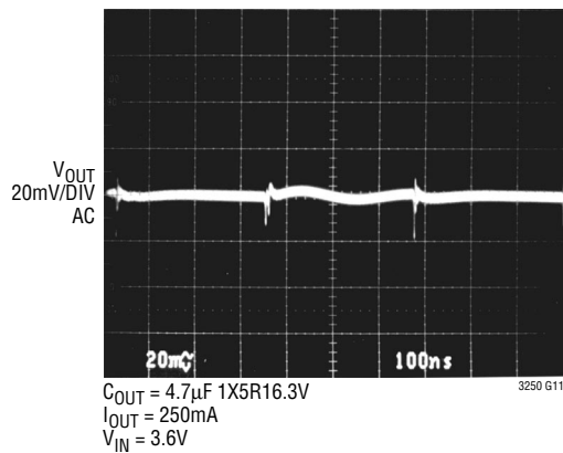
Output Voltage Ripple (LTC3250-1.5)
