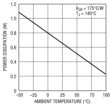
Figure 3. Maximum Power Dissipation vs Ambient Temperature
