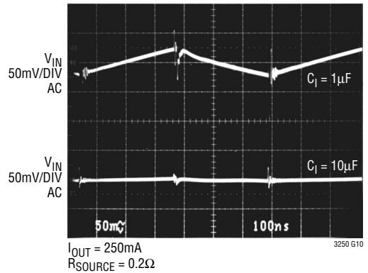
Input Voltage Ripple vs Input Capacitor (LTC3250-1.5)
