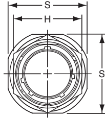
TERMINATION ASSEMBLIES "SE" (SR), MS/"F" Strain Relief
