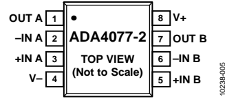
Figure 8. ADA4077-2 Pin Configuration, 8-Lead SOIC
