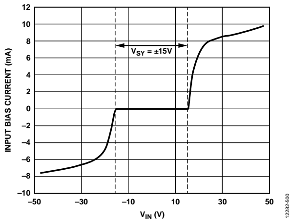
Figure 88. Input Bias Current During Positive and Negative Overvoltage, V_{SV} = \pm 15\text{ V} , Voltage Follower Configuration
