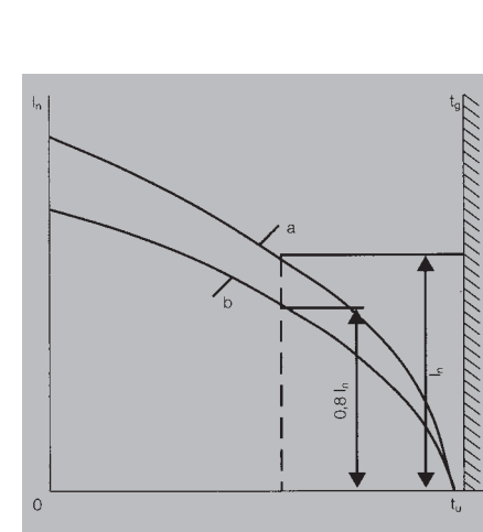
Derating curve
