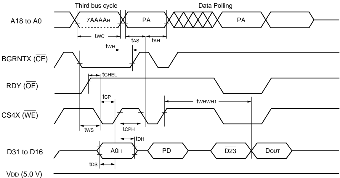
c : Write data polling read ( \overline{CE} control)
