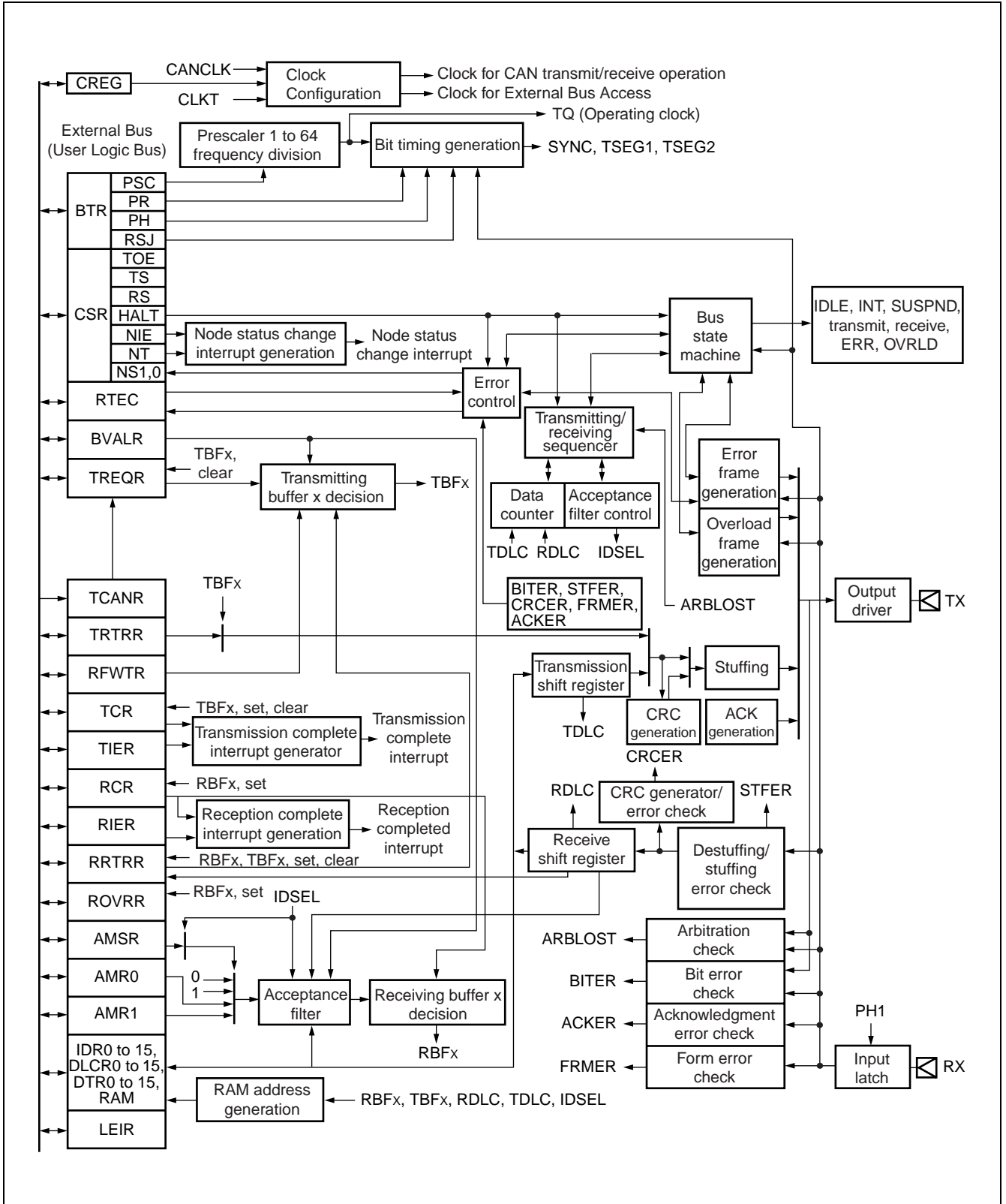
(3) Block diagram
