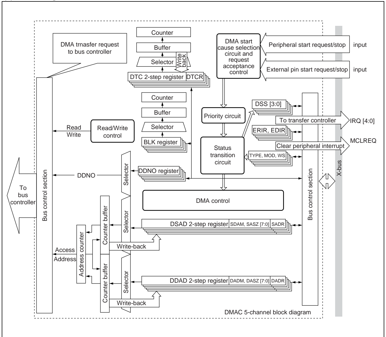
(4) Block diagram
