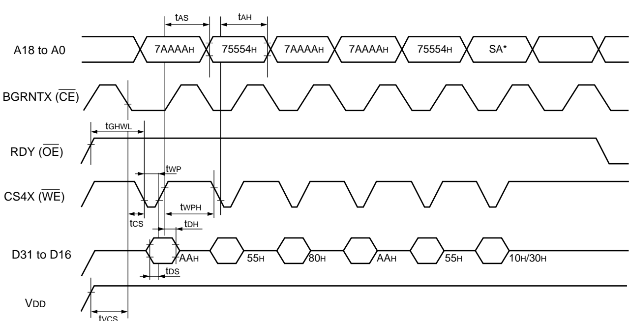
d : Chip erase/sector erase command sequence
