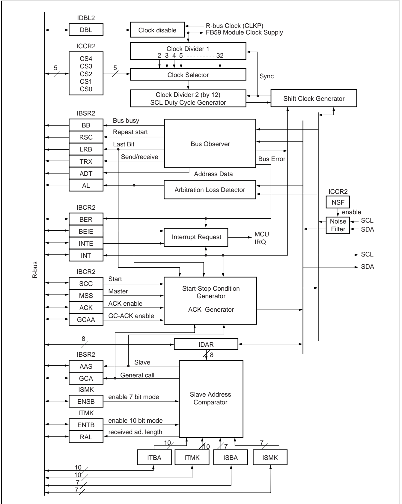
(2) Block diagram
