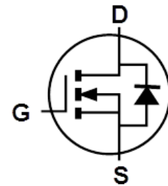
Internal Schematic
