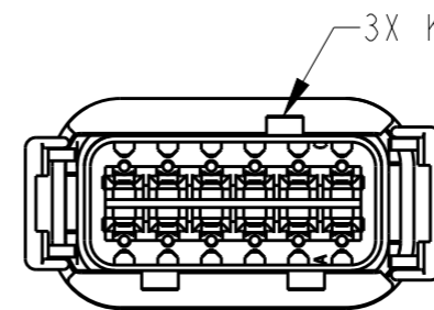
DTM04-12PC-E005 KEY -C-
