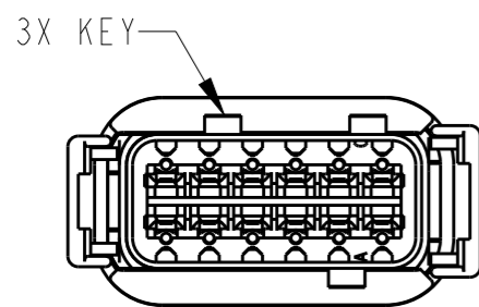
DTM04-12PA-E005 KEY -A-
