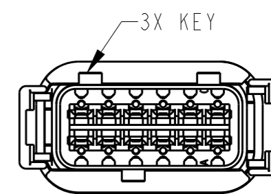
DTM04-12PD-E005 KEY -D-
