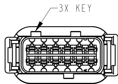
DTM04-12PB-E005 KEY -B-
