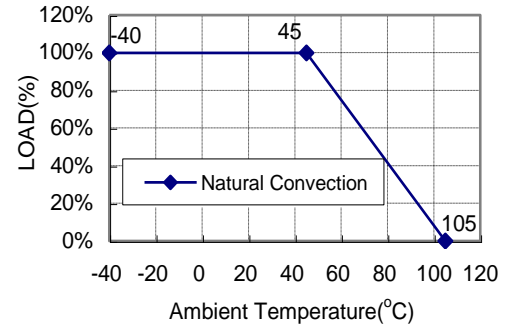
Typical Derating Curve
