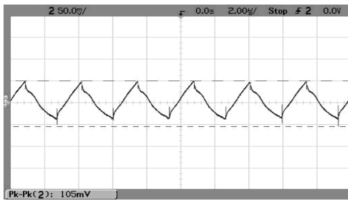
Output Ripple and Noise (Vin=12V, Vout=5V, Iout=16A, Clad=0, ScopeBW=100MHz)
