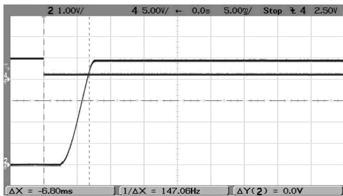
On/Off Enable Startup Delay (Vin=8.3V, Vout=5V, Iout=16A, Clad=0) Trace 4=Enable In, Trace2=Vout
