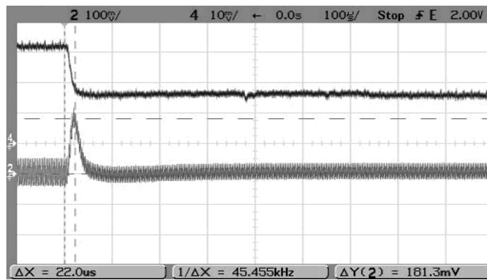
Step Load Transient Response (Vin=12V, Vout=5V, Clad=0, Iout=16A to 8A) Trace 2=Vout, 100 mV/div, Trace4=Iout, 5A/div.
