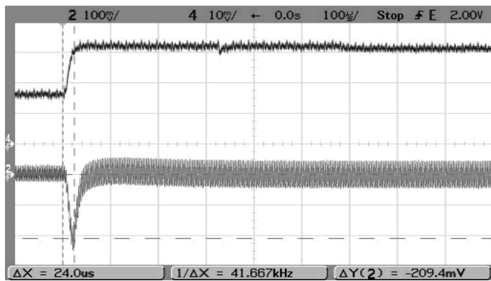
Step Load Transient Response (Vin=12V, Vout=5V, Clad=0, Iout=8A to 16A) Trace 2=Vout, 100 mV/div, Trace4=Iout, 5A/div.
