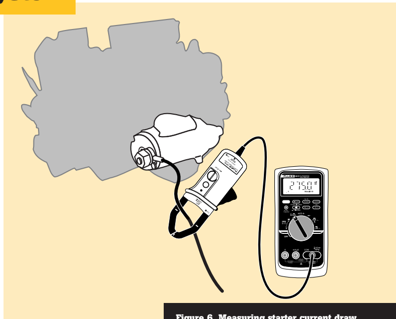
Figure 6. Measuring starter current draw
