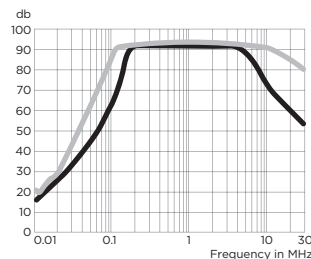
36FCD10B
