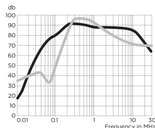
150FCD10BS
