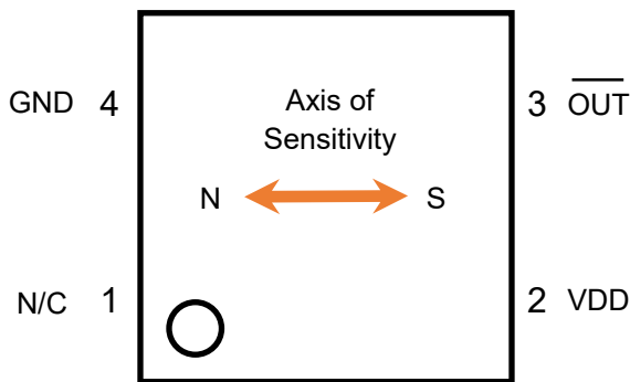
LGA Package for CT832
