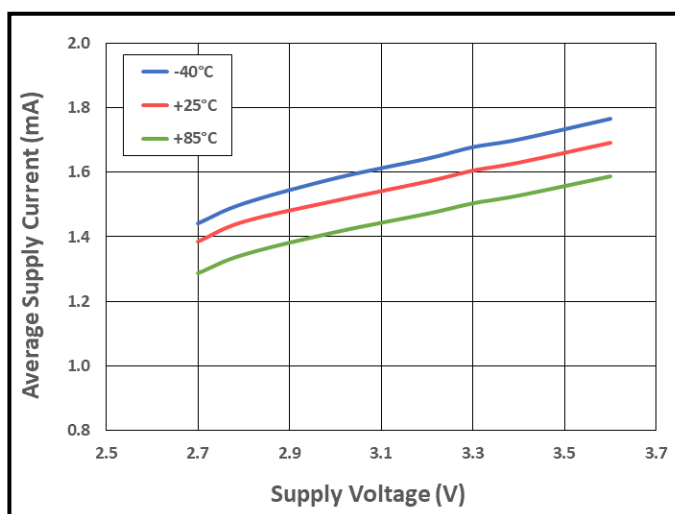
Figure 17. Average Supply Current vs. Supply Voltage vs. Temperature
