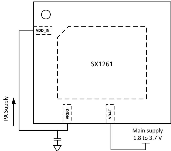
Figure 5-2: SX1261 Diagram with the LDO Regulator Power Option
