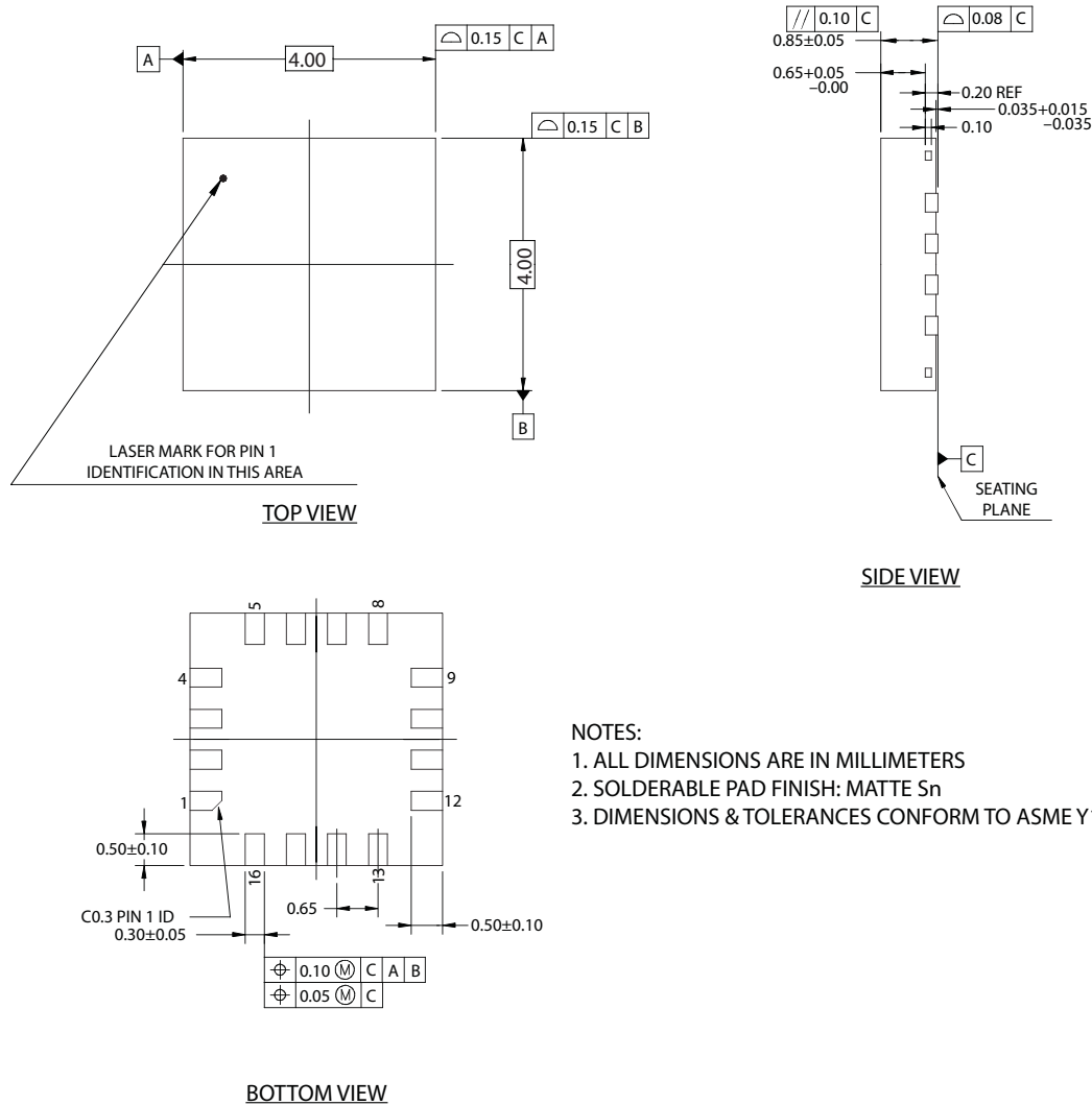
Figure 7-1: Package Dimensions
