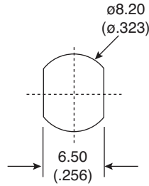
MOUNT HOLE
