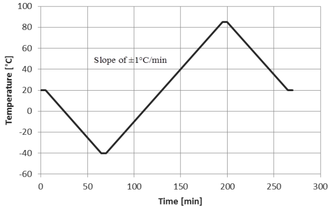
Figure 26: Recommended Temperature profile for calibration
