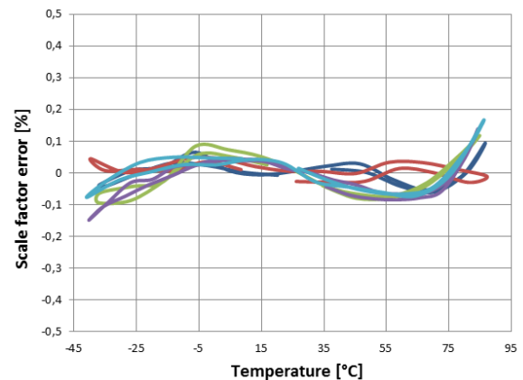
Figure 5 Scale factor variation over temperature (5 samples)
