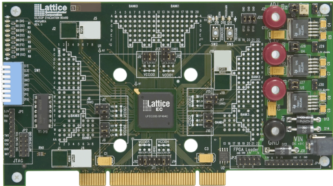
Figure 1. LatticeEC Standard Evaluation Board
