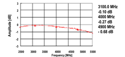
Amplitude Balance
