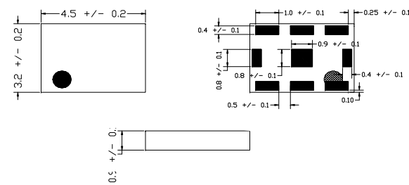
[MECHANICAL DIMENSIONS]
