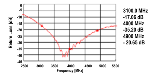
Return Loss [dB]
