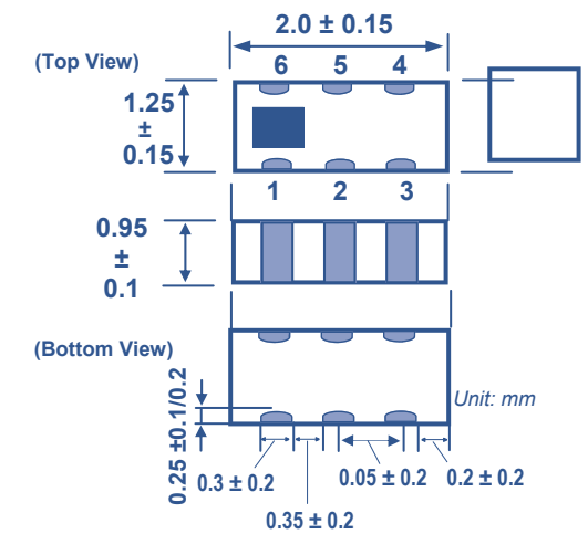
Mechanical Dimensions
