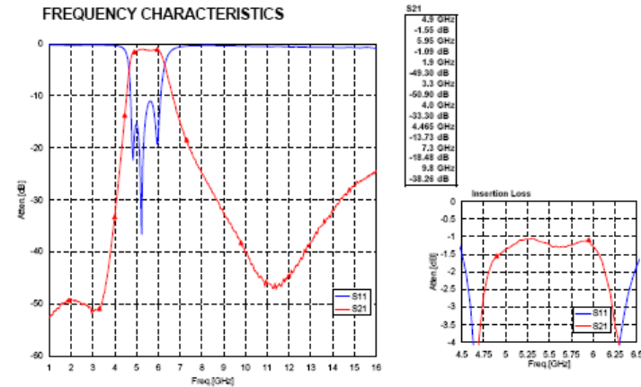
FREQUENCY CHARACTERISTICS
